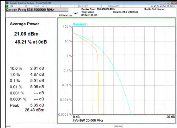
B5_1_QPSK_Middle_
