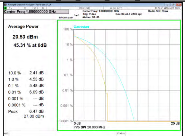
B2_100_QPSK_Middle_
