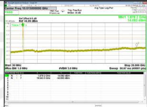
16QAM_20M_Higher_Conducted Spurious
