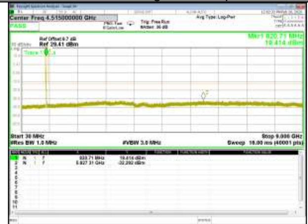
B26_Q16_5M_High_CDT_Spurious
