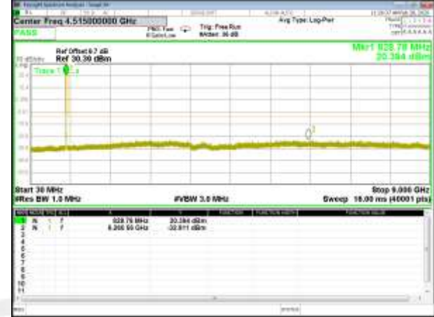
B5_Q16_5M_Mid_CDT_Spurious
