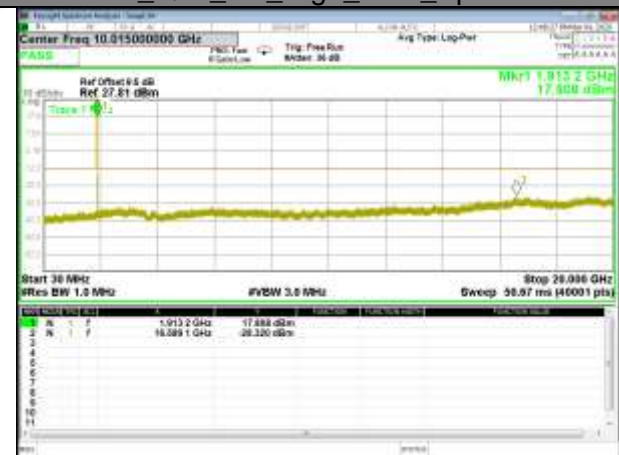
B25_Q16_3M_High_CDT_Spurious
