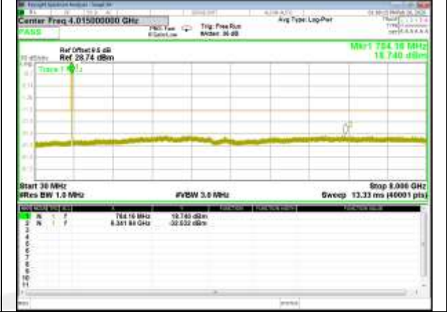
B13_Q16_10M_Mid_CDT_Spurious
