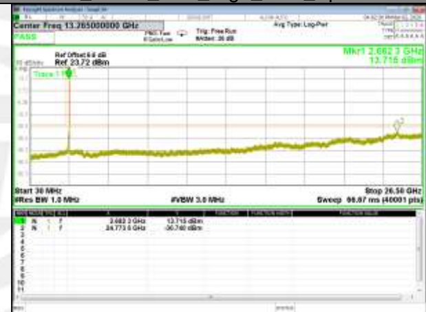
B41_Q16_20M_High_CDT_Spurious
