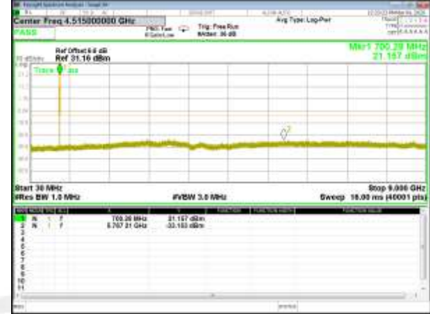
B12_Q16_1.4M_Mid_CDT_Spurious
