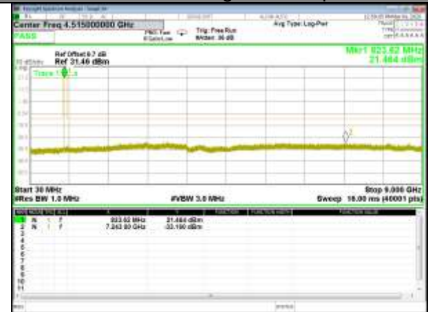
B26_Q16_1.4M_High_CDT_Spurious
