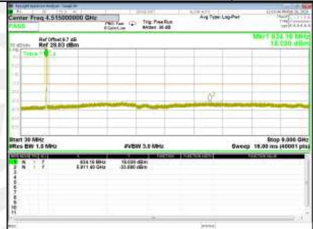
B26_Q16_10M_High_CDT_Spurious
