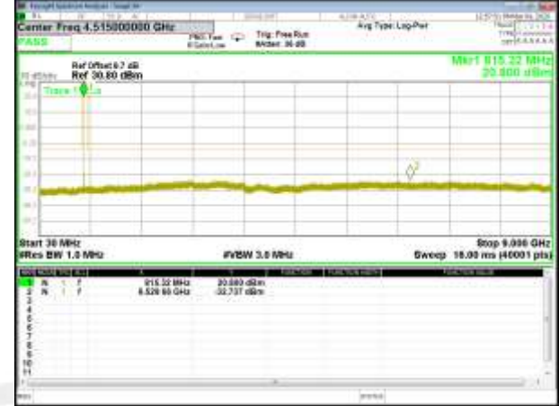
B26_Q16_1.4M_Mid_CDT_Spurious
