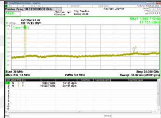
16QAM_15M_Higher_Conducted Spurious
