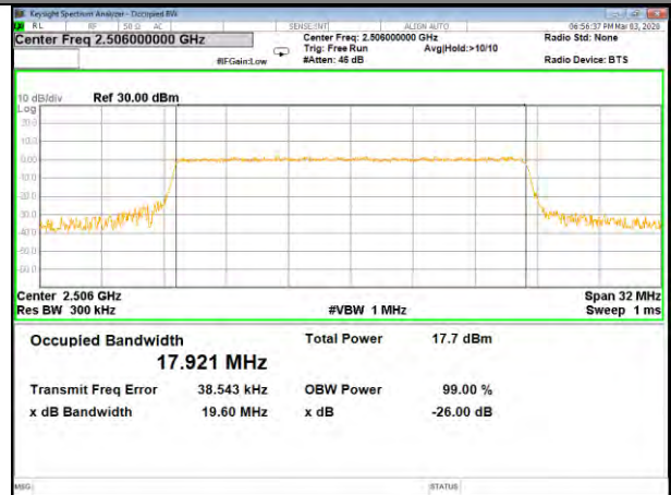
B41_Q16_20M_Low_26BW-99%
