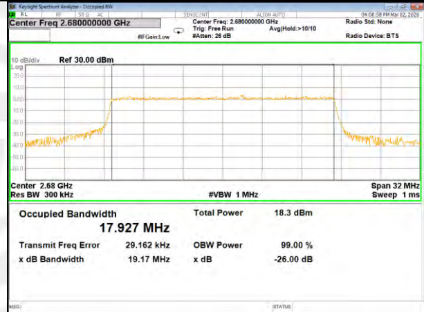
B41_Q16_20M_High_26BW-99%
