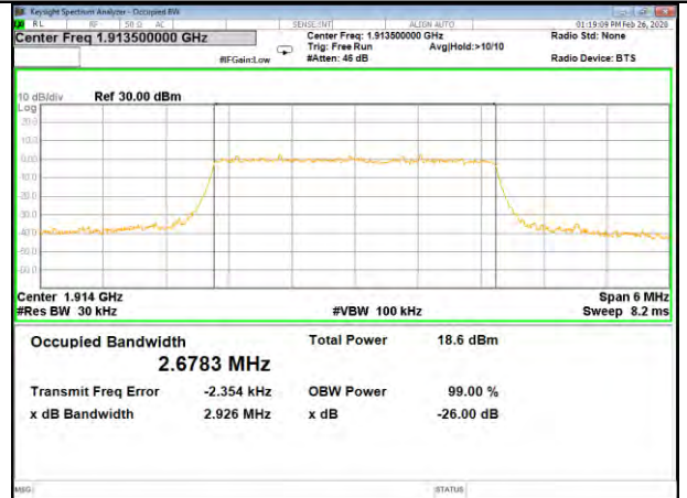
B25_Q16_3M_High_26BW-99%
