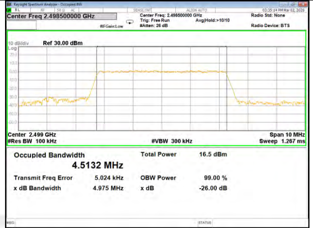
B41_Q16_5M_Mid_26BW-99%
