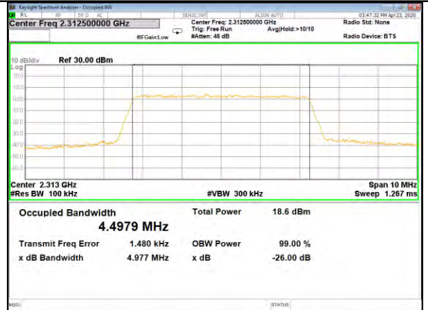
B30_Q16_5M_High_26BW-99%
