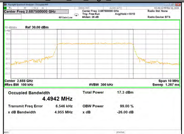
B41_Q16_5M_High_26BW-99%
