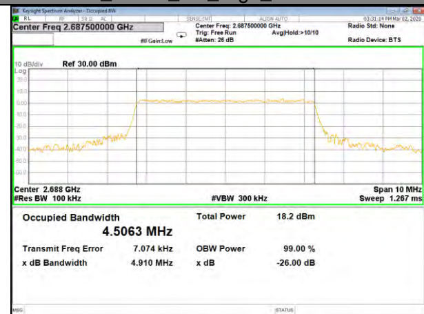
B41_QPSK_5M_High_26BW-99%
