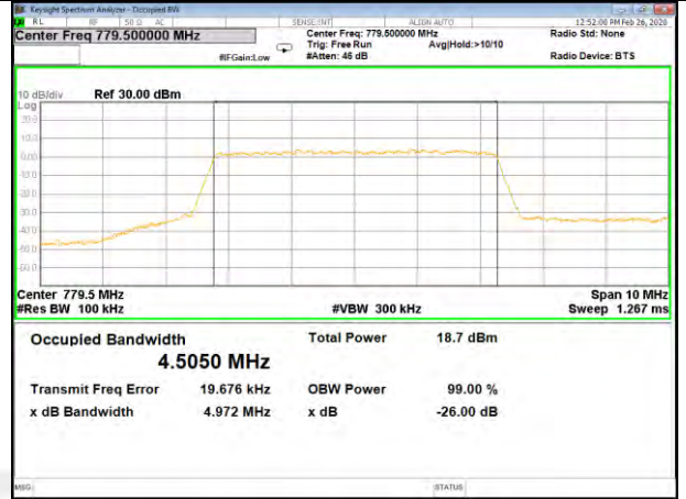
B13_Q16_5M_Mid_26BW-99%
