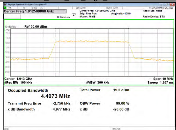
B25_Q16_5M_High_26BW-99%
