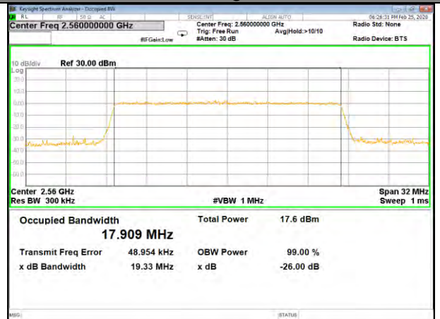
B7_Q16_20M_High_26BW-99%
