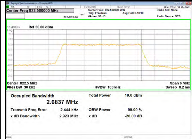
B26_QPSK_3M_High_26BW-99%
