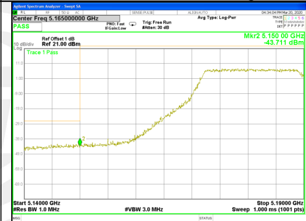
W52_11ac80_CH42(5210MHz)_Conducted Spurious
