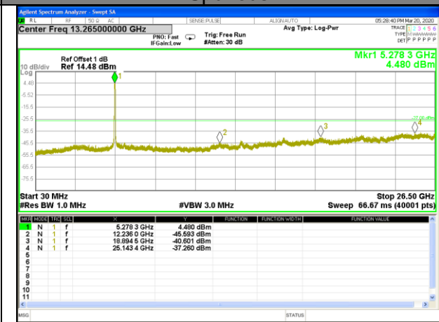
W53_11ac80_CH58(5290MHz)_Conducted Spurious
