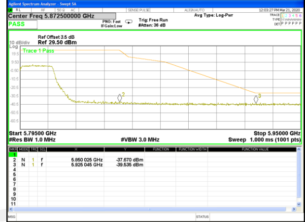
W58_11ac20_Middle_Conducted Spurious
