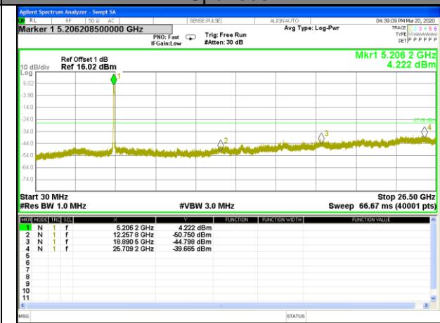
W52_11ac80_CH42(5210MHz)_Conducted Spurious
