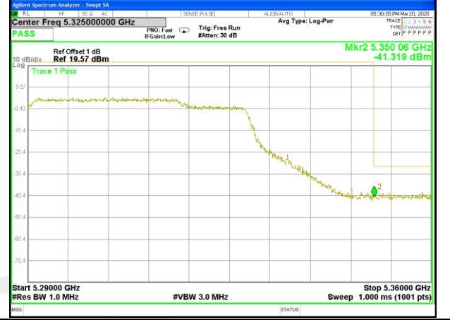
W53_11ac80_CH58(5290MHz)_Band edge_Right
