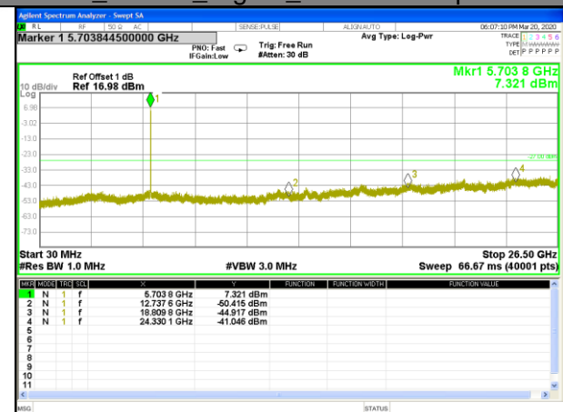
W56_11ac20_Higher_Conducted Spurious
