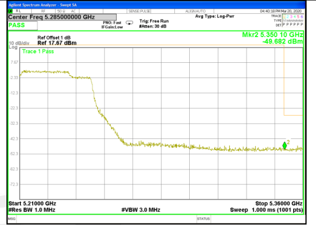
W52_11ac80_CH42(5210MHz)_Band edge_Right
