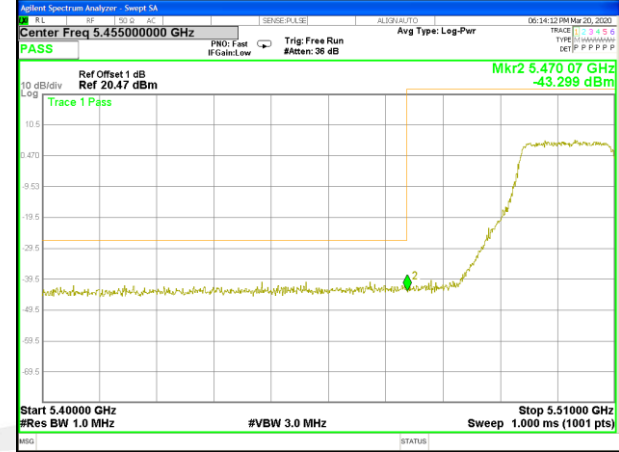
W56_11ac20_Lower_Conducted Spurious
