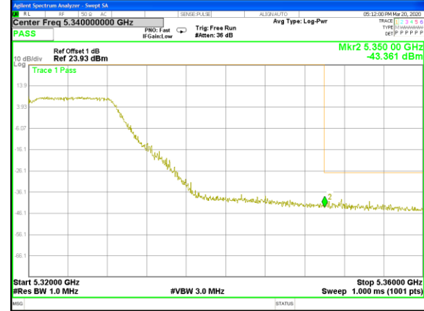
W53_11ac40_Higher_Conducted Spurious
