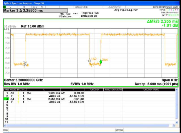
Band 1-n20-Ant A
