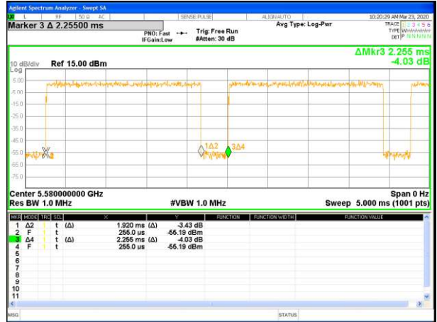
Band 3-n20-Ant A
