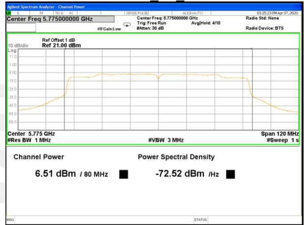
5775MHz_AV_Ant B
