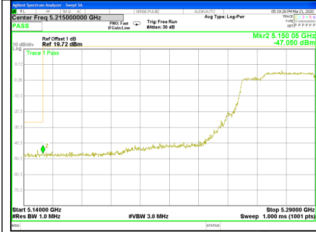
W53_11ac80_CH58(5290MHz)_Band edge_left
