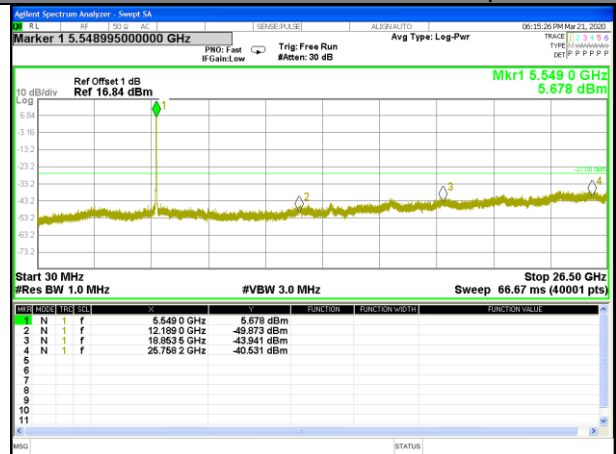
W56_11n40_Middle_Conducted Spurious
