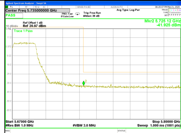
W56_11ac20_Middle_Conducted Spurious
