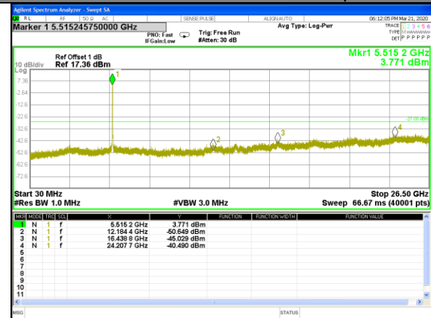
W56_11n40_Lower_Conducted Spurious
