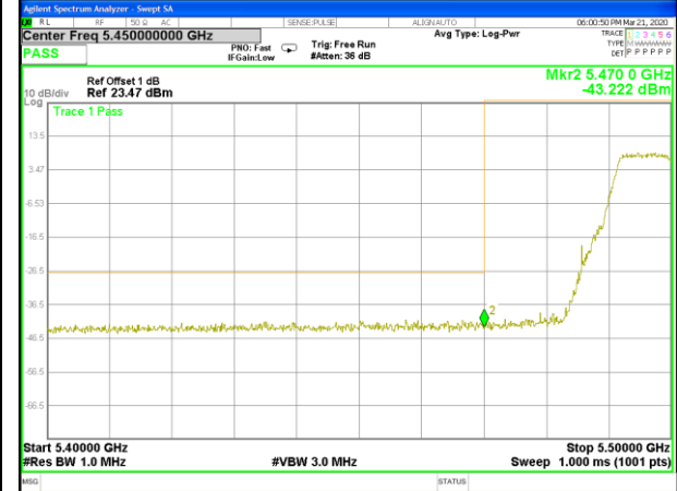
W56_11ac40_Lower_Conducted Spurious
