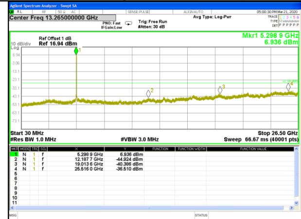
W53_11n40_Higher_Conducted Spurious
