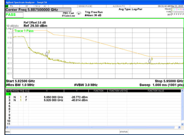
W58_11ac40_Higher_Conducted Spurious
