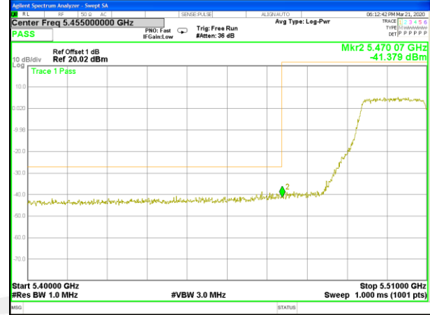
W56_11ac20_Lower_Conducted Spurious
