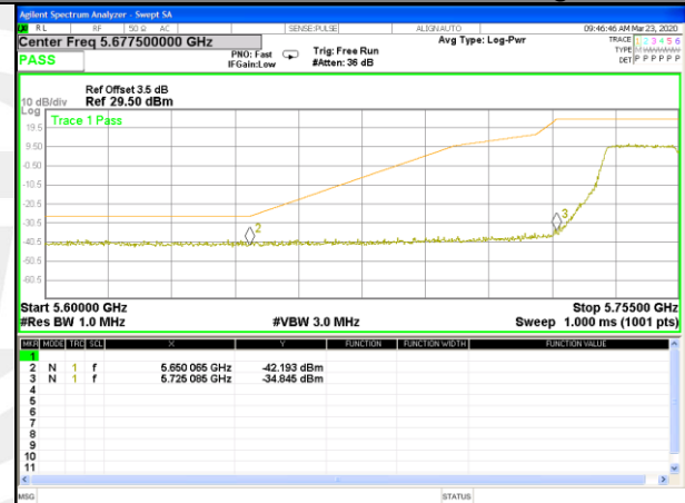
W58_11ac80_Spurious_30M26BWG_5775M
