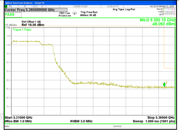
W52_11ac80_CH42(5210MHz)_Band edge_Right
