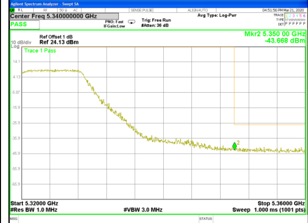
W53_11ac40_Higher_Conducted Spurious
