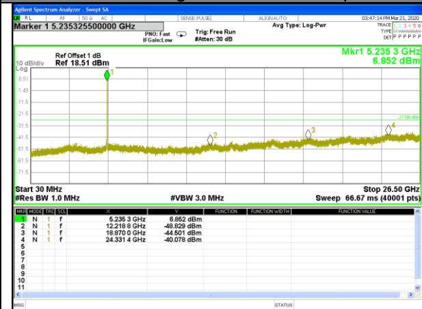
W52_11ac20_Higher_Conducted Spurious
