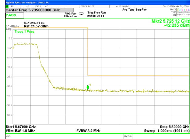
W56_11ac80_Higher_Conducted Spurious
