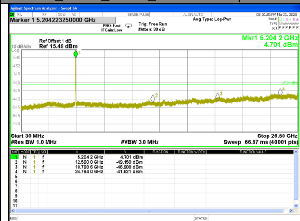
W52_11n40_Lower_Conducted Spurious
