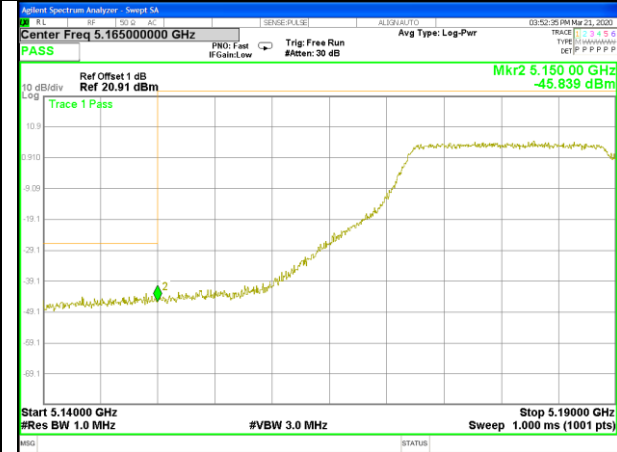
W52_11ac20_Lower_Conducted Spurious
