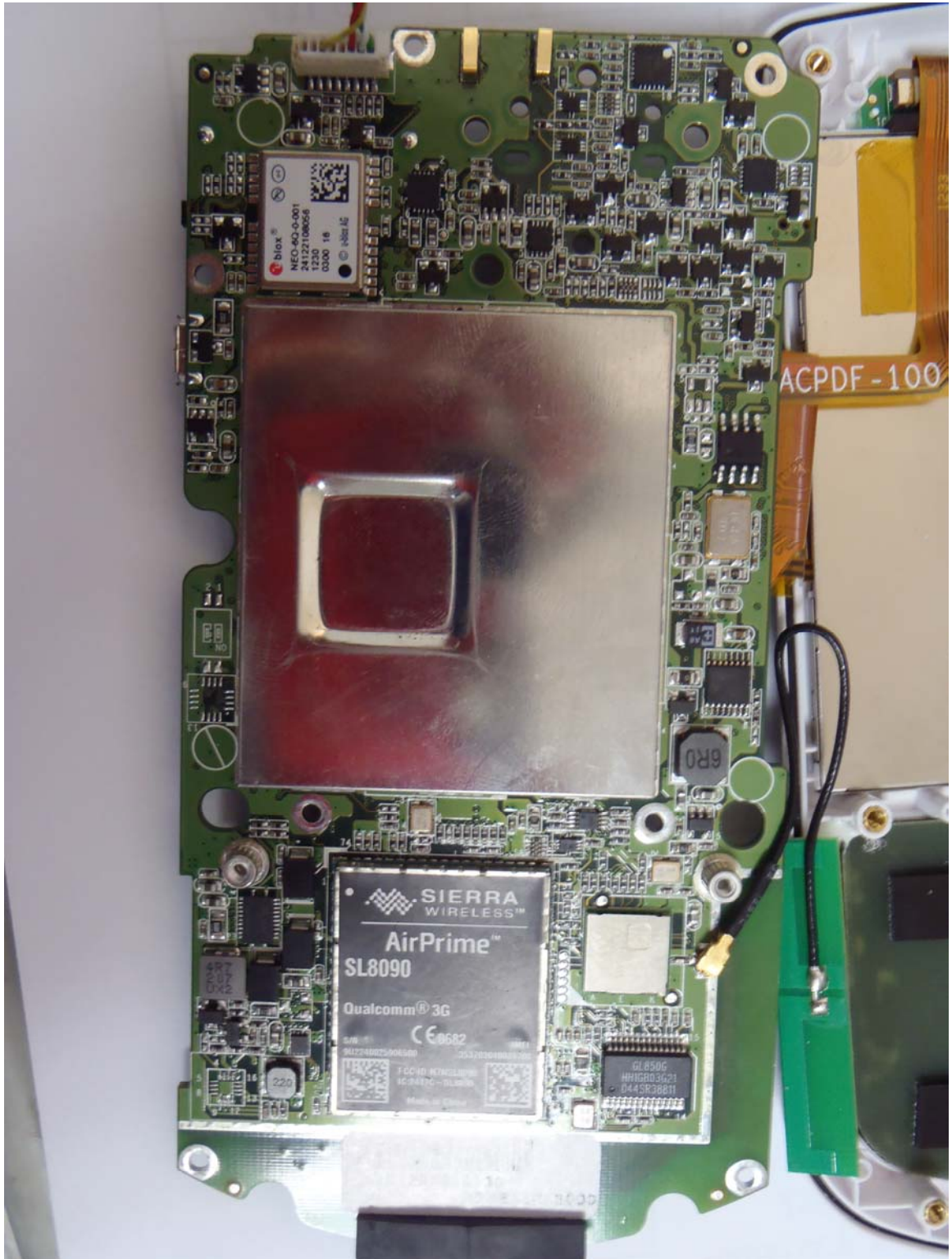
EUT inside Front View
