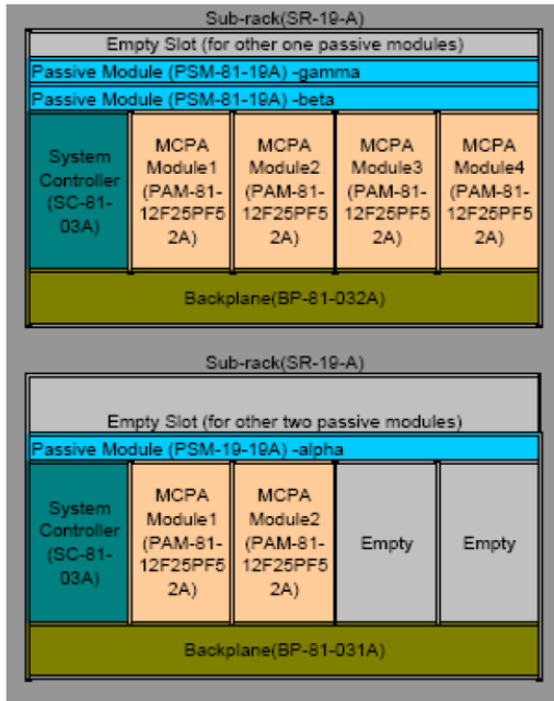
Configuration 3 - 850 MHz, 4x2, 3 sector TS-81-1203354A
