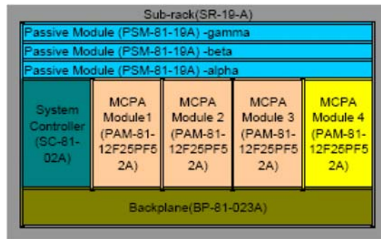
Configuration 2 - 850 MHz, N+1, 3 sector TS-81-1202351A
