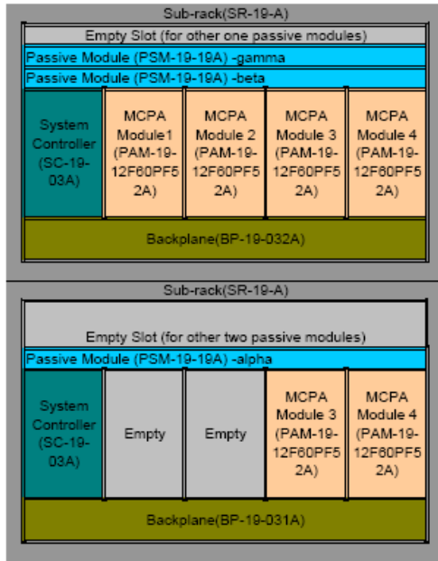
Configuration 9 - 1900 MHz, 4x2, 3 sector TS-19-1203354A
