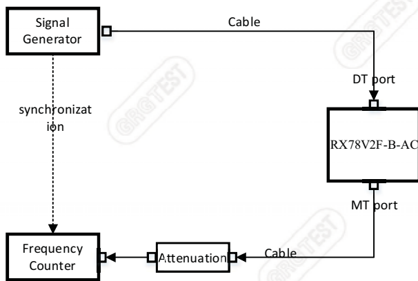
Figure 12.10-1 Downlink connection diagram
