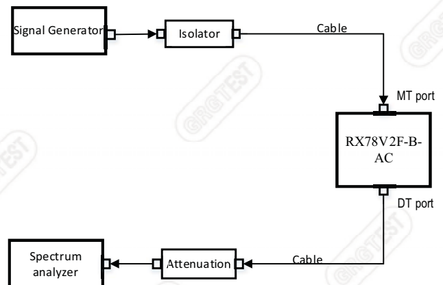
Figure 12.9-2 Uplink connection diagram
