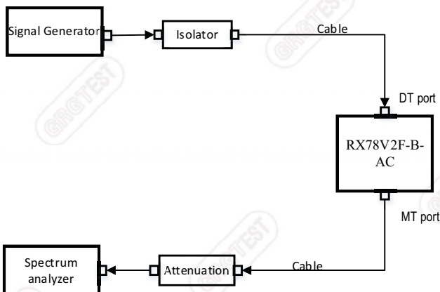
Figure 12.9-1 Downlink connection diagram
