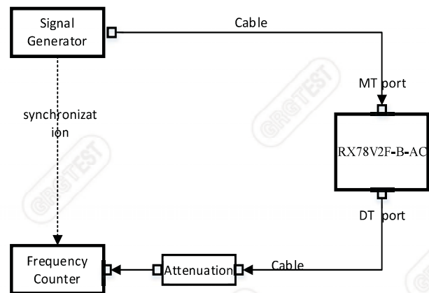
Figure 12.10-2 Uplink connection diagram
