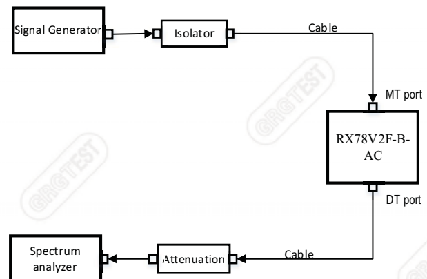
Figure 12.5-2 Uplink connection diagram
