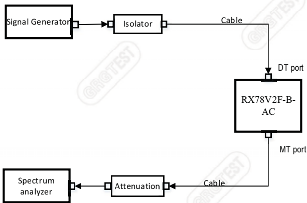
Figure 12.5-1 Downlink connection diagram
