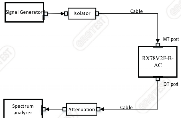
Figure 12.4-2 Uplink connection diagram
