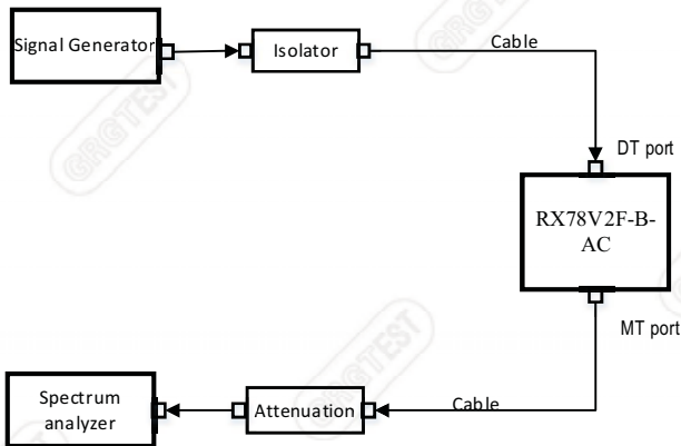
Figure 12.4-1 Downlink connection diagram
