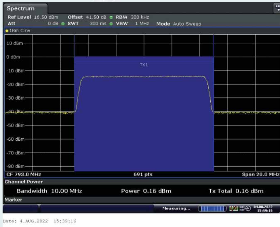
Middle Frequency: 793.0MHz, Input occupied BW
