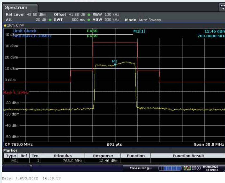
With the input signal amplitude set 3 dB above the AGC threshold Middle Frequency: 763.0MHz
