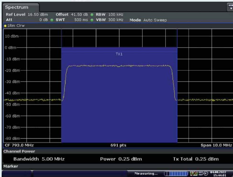
Middle Frequency: 793.0MHz, Input occupied BW
