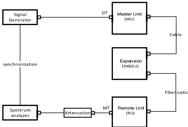
Figure 11.4-1 Downlink connection diagram
