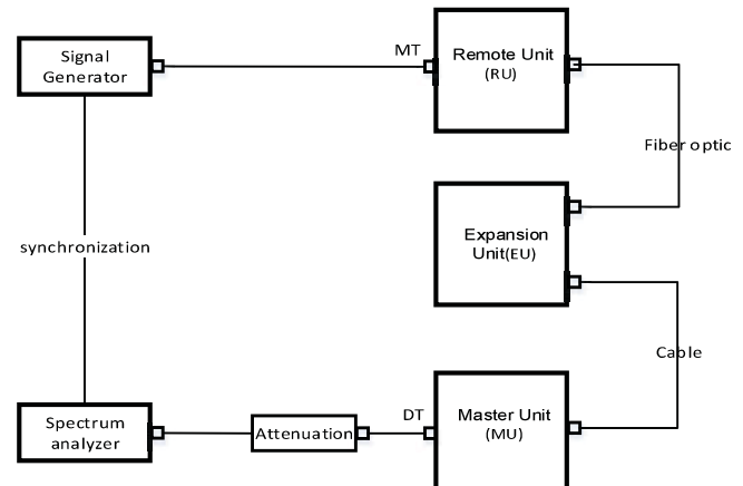
Figure 11.4-2 Uplink connection diagram
