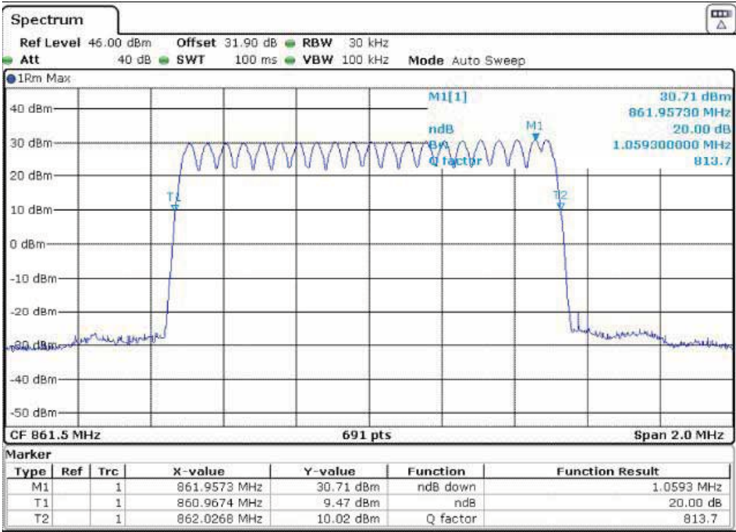
Downlink: 861MHz~862MHz
