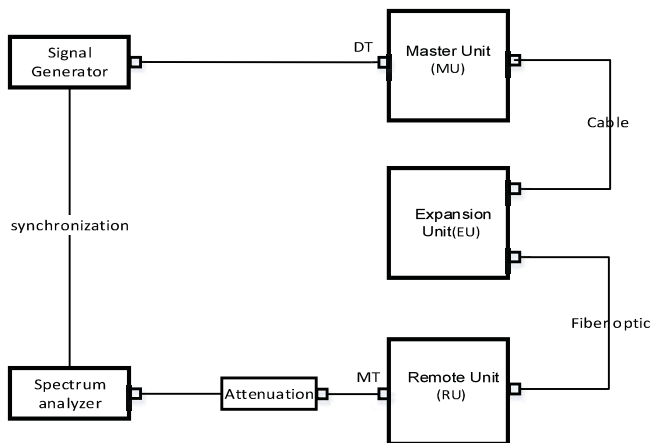
Figure 11.5-1 Downlink connection diagram
