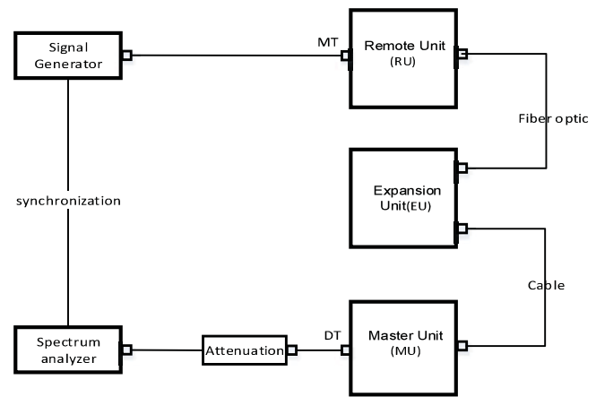
Figure 11.5-2 Uplink connection diagram
