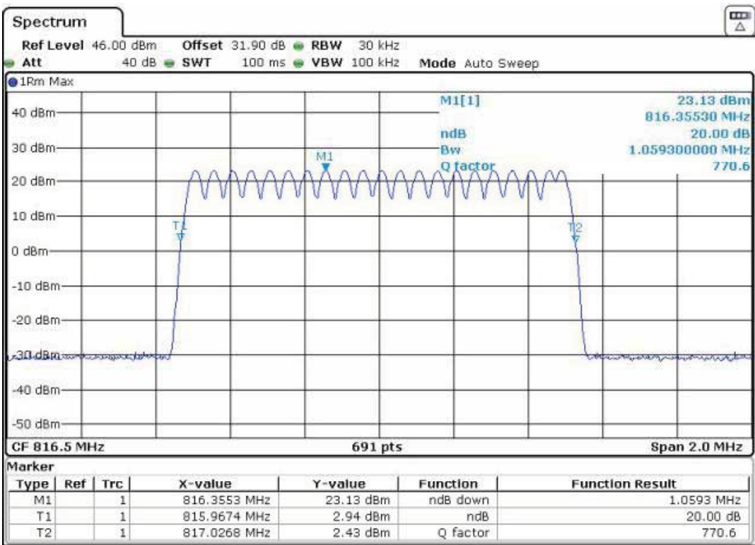
Uplink: 816MHz~817MHz
