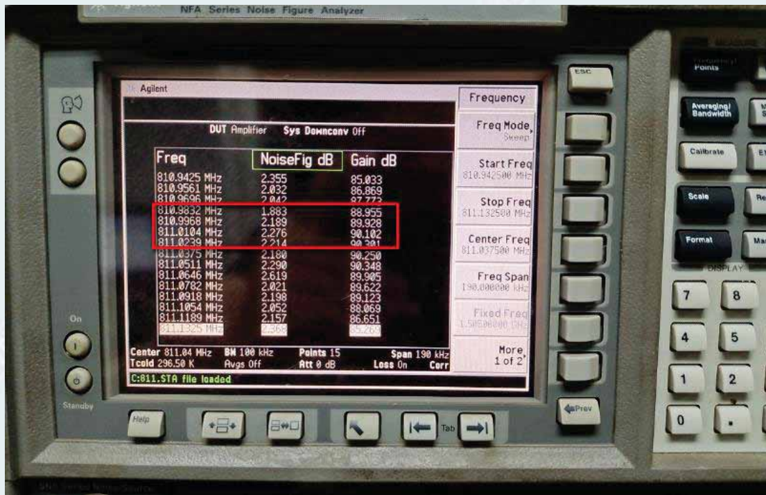
Middle frequency: 811.0MHz
