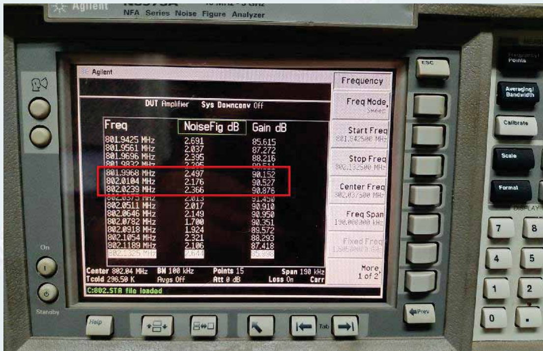
Middle frequency: 802.0MHz
