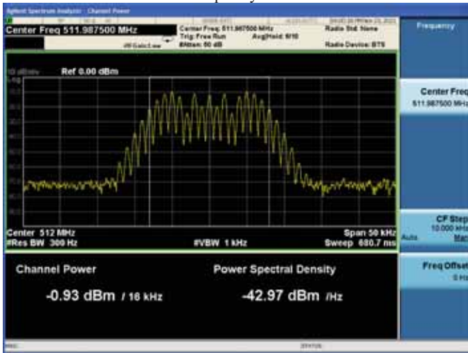
Input signal High Frequency: 511.9875MHz
