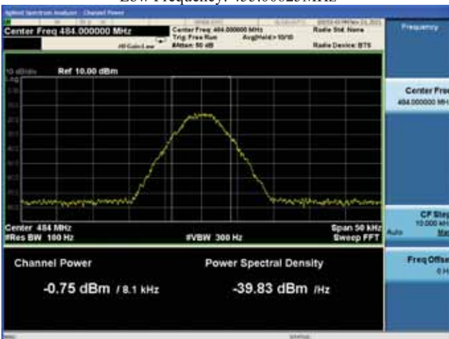
Input signal
