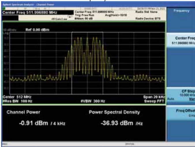
Input signal High Frequency: 511.99688MHz
