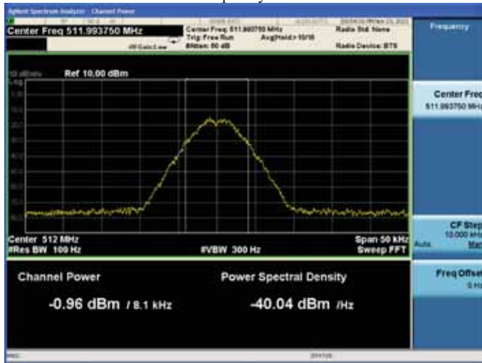
Input signal High Frequency: 511.99375MHz
