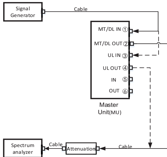
Figure 10.4-1 MU single device test connection diagram
