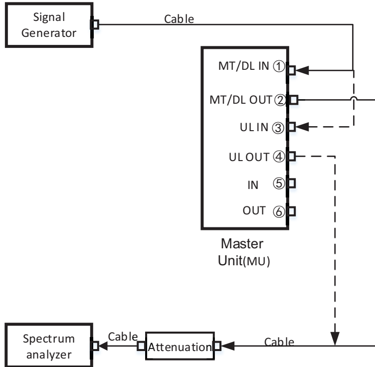
Figure 1 MU single device test connection diagram
