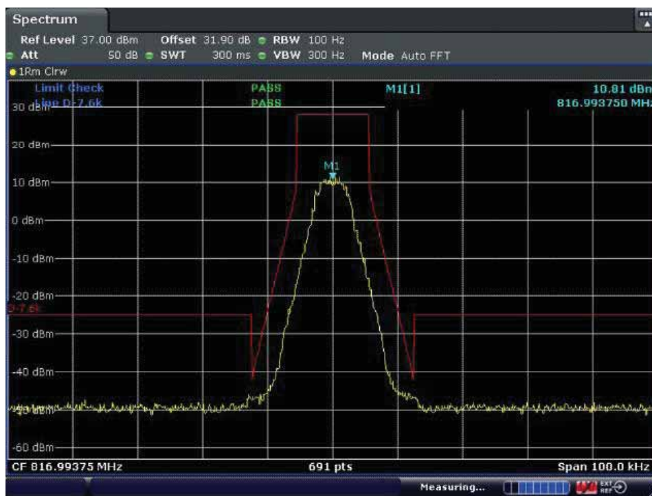
With the input signal amplitude set 3 dB above the AGC threshold Highest Frequency: 816.99375MHz
