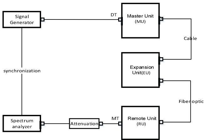
Figure 11.5-1 Downlink connection diagram
