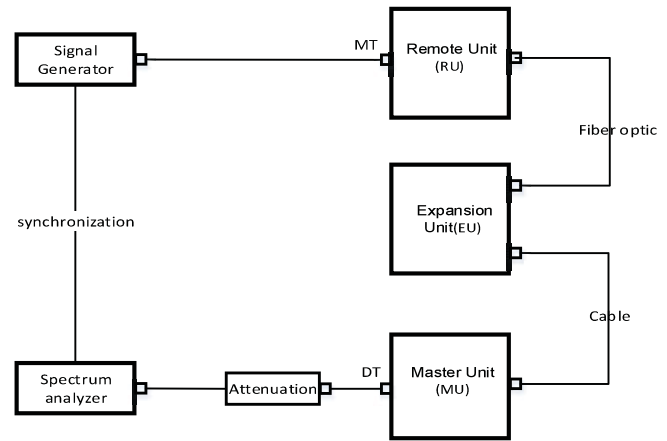
Figure 11.4-2 Uplink connection diagram
