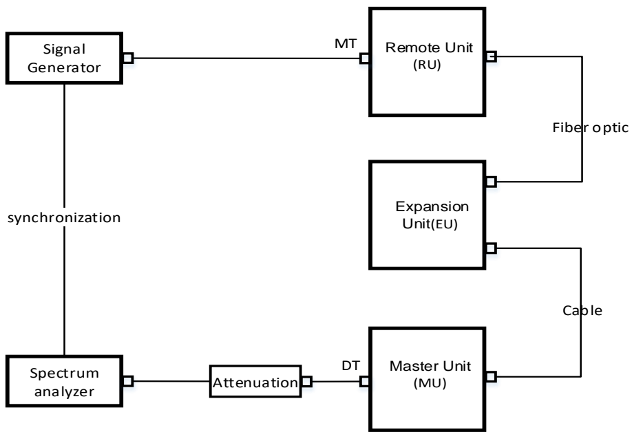
Figure 11.5-2 Uplink connection diagram
