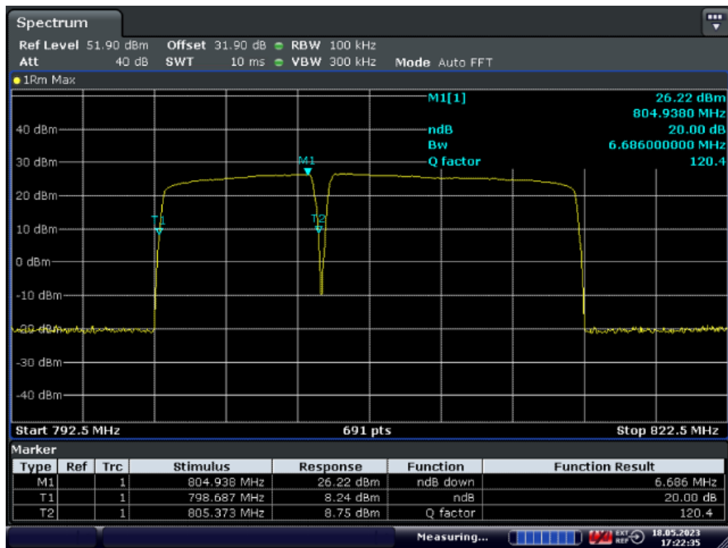
Uplink: 799MHz~805MHz
