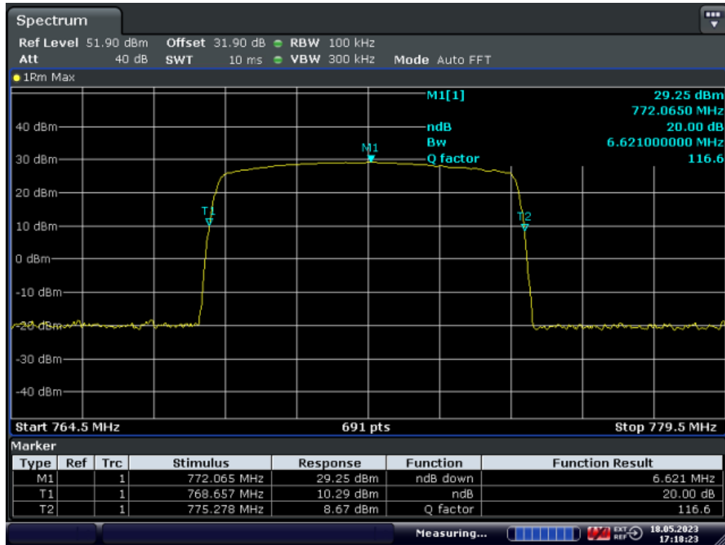
Downlink: 769MHz~775MHz
