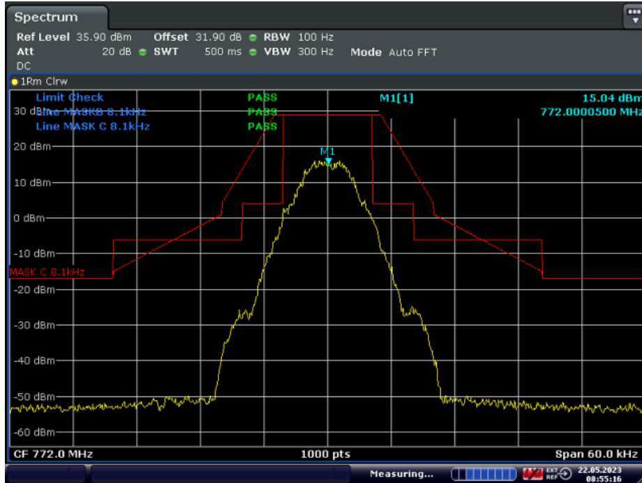
With the input signal amplitude set the AGC threshold Middle Frequency: 772.0MHz
