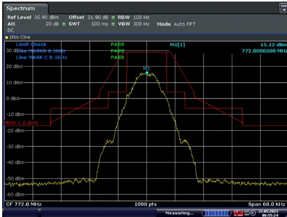
With the input signal amplitude set 3 dB above the AGC threshold Middle Frequency: 772.0MHz
