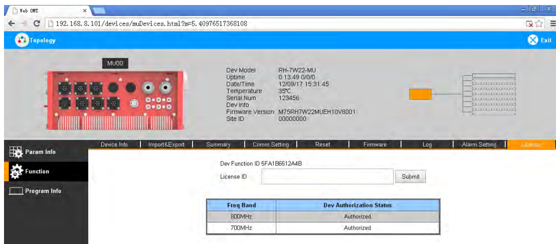
Figure 38: Function – License
