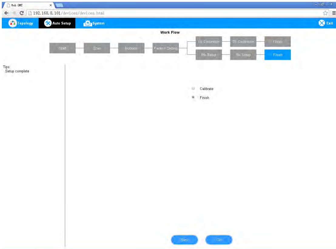
Figure 46: Finish
