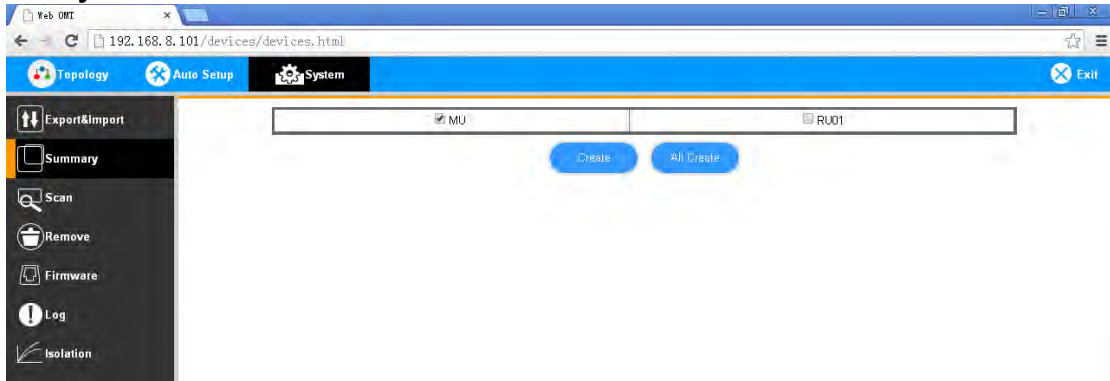
Figure 48: System – Summary
