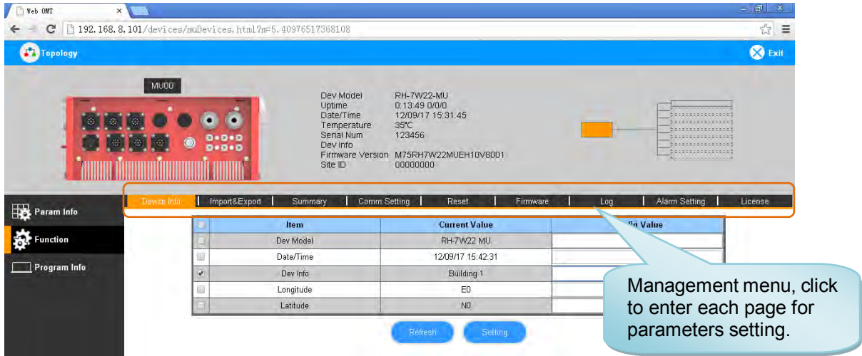
Figure 29: [Function] Screen
