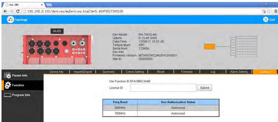
Figure 38: Function – License
