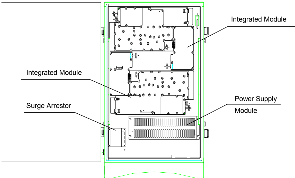
Figure 7: Layout of the RU Bottom layer
