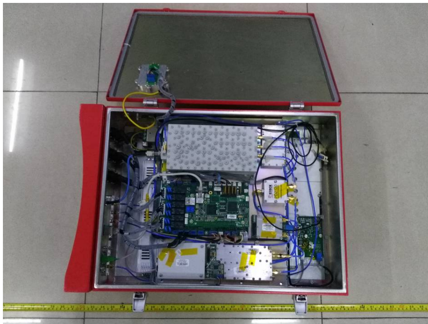
EUT – Cover off View 4 (Model: RH-7W22-R-AC)
