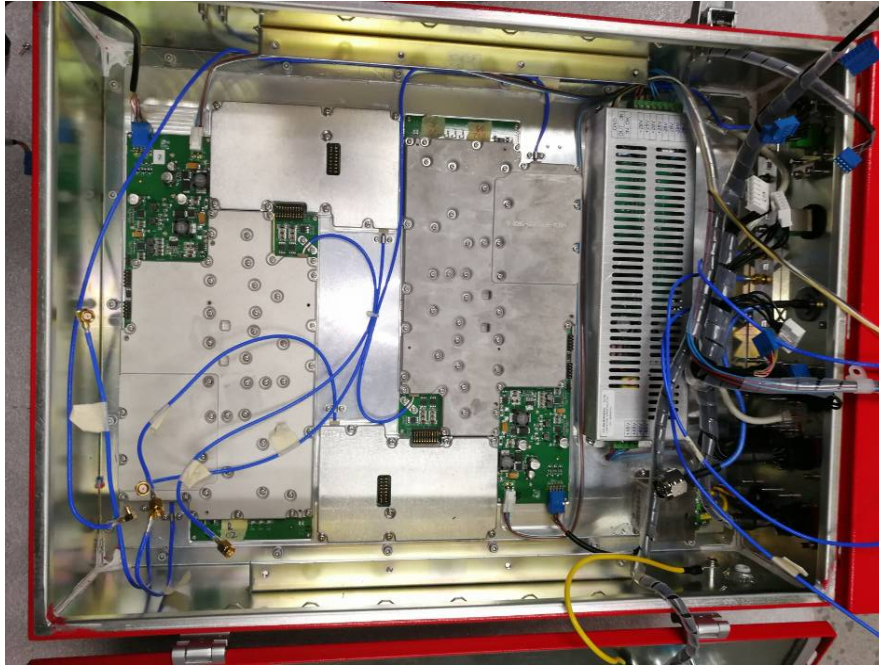
EUT – Cover off View 3 (Model: RH-7W22-R)
