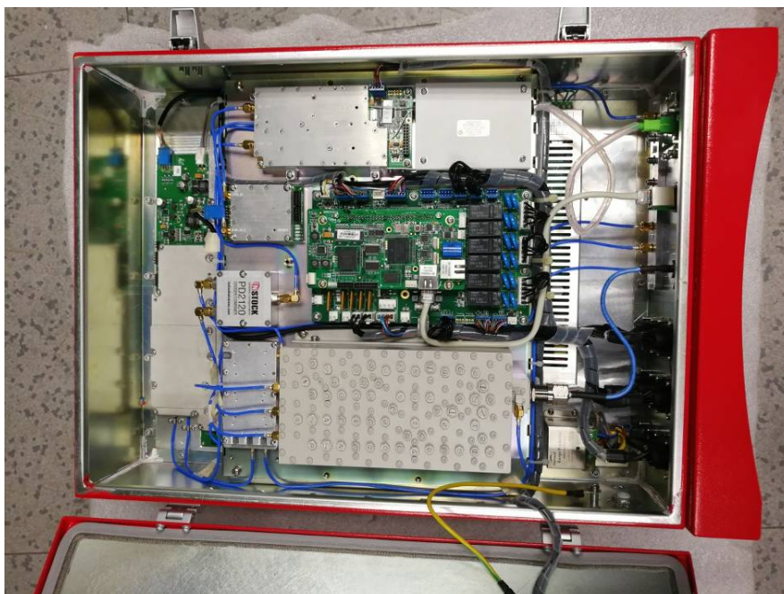
EUT – Cover off View 1 (Model: RH-7W22-R)
