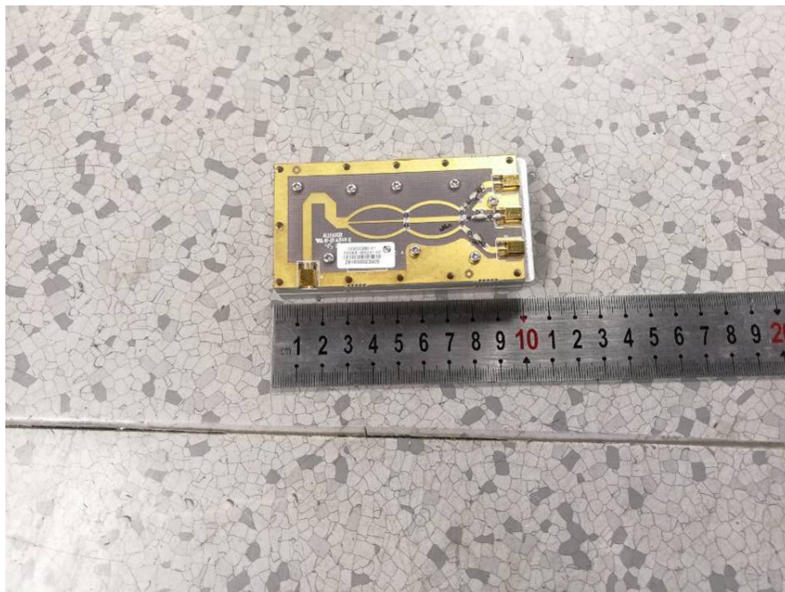
EUT – Splitter Module 1 Board View
