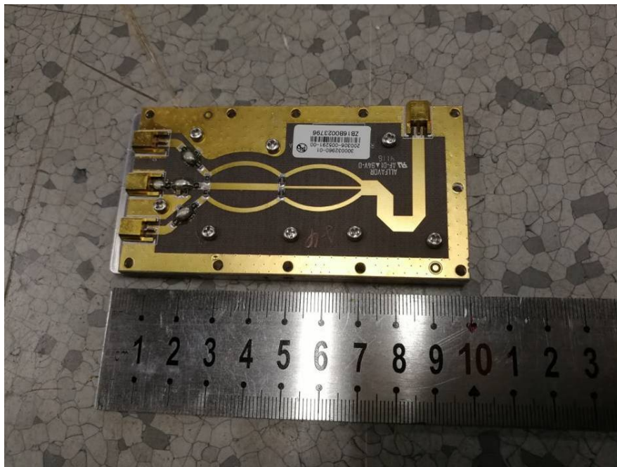
EUT – Splitter Module 2 Board View
