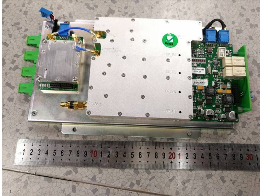
EUT – Adapter Module View
