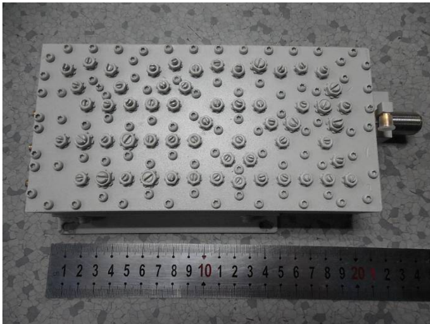
EUT – Duplexer Module View 1
