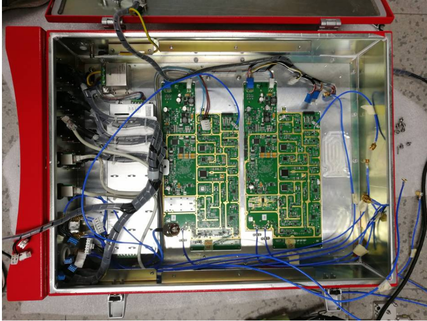
EUT – Cover off View 5 (Model: RH-7W22-D)
