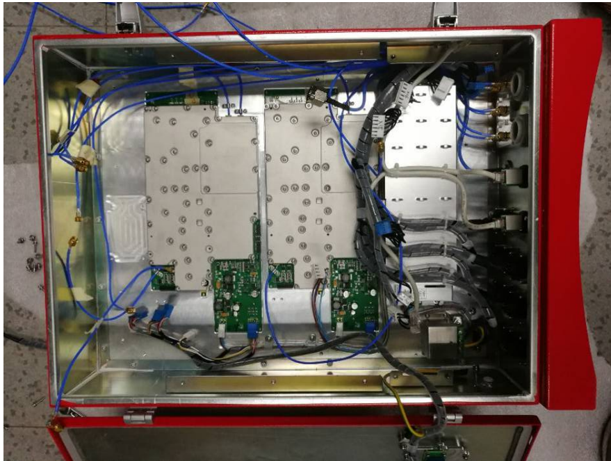
EUT – Cover off View 4 (Model: RH-7W22-D)
