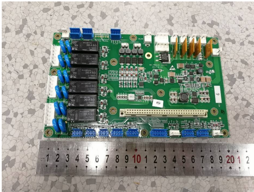
EUT – Distribution Board Top View
