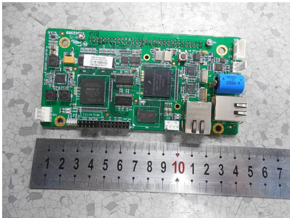
EUT – MCU Board Top View
