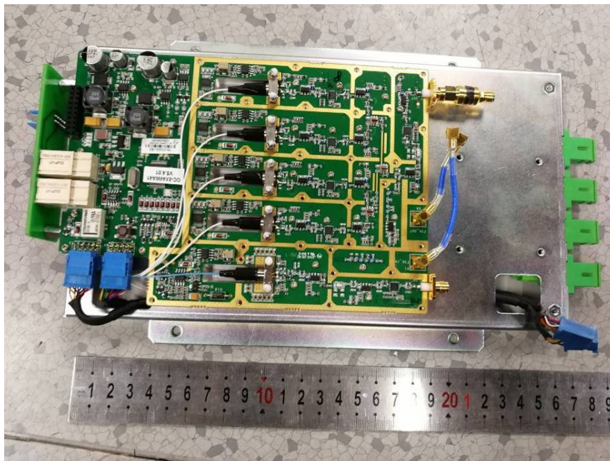
EUT – Optical Module Top View
