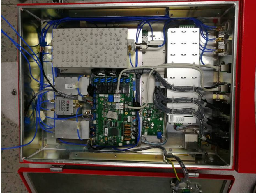
EUT – Cover off View 3 (Model: RH-7W22-D)
