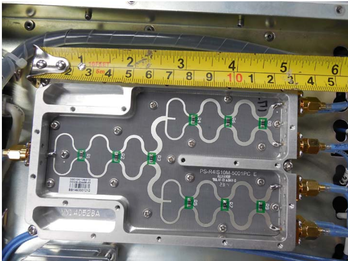
(14)MU Combiner
