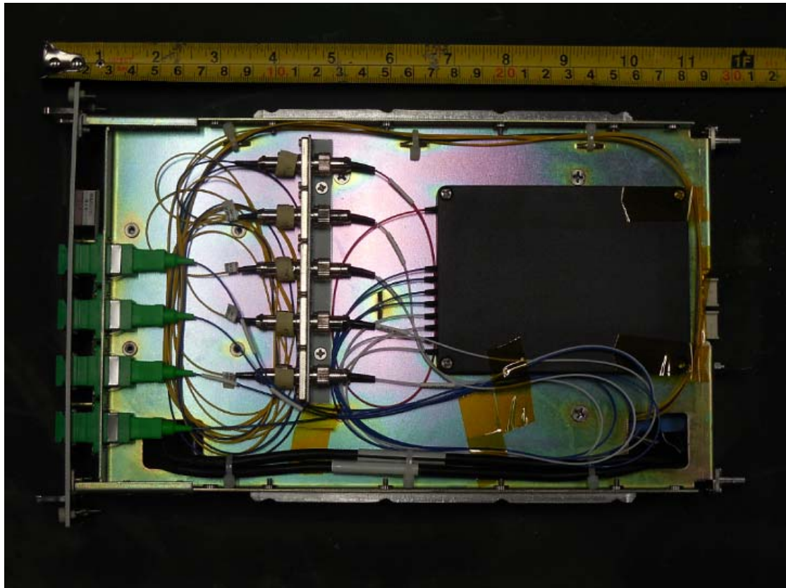
(6) MU01-RFU-7LB181D
