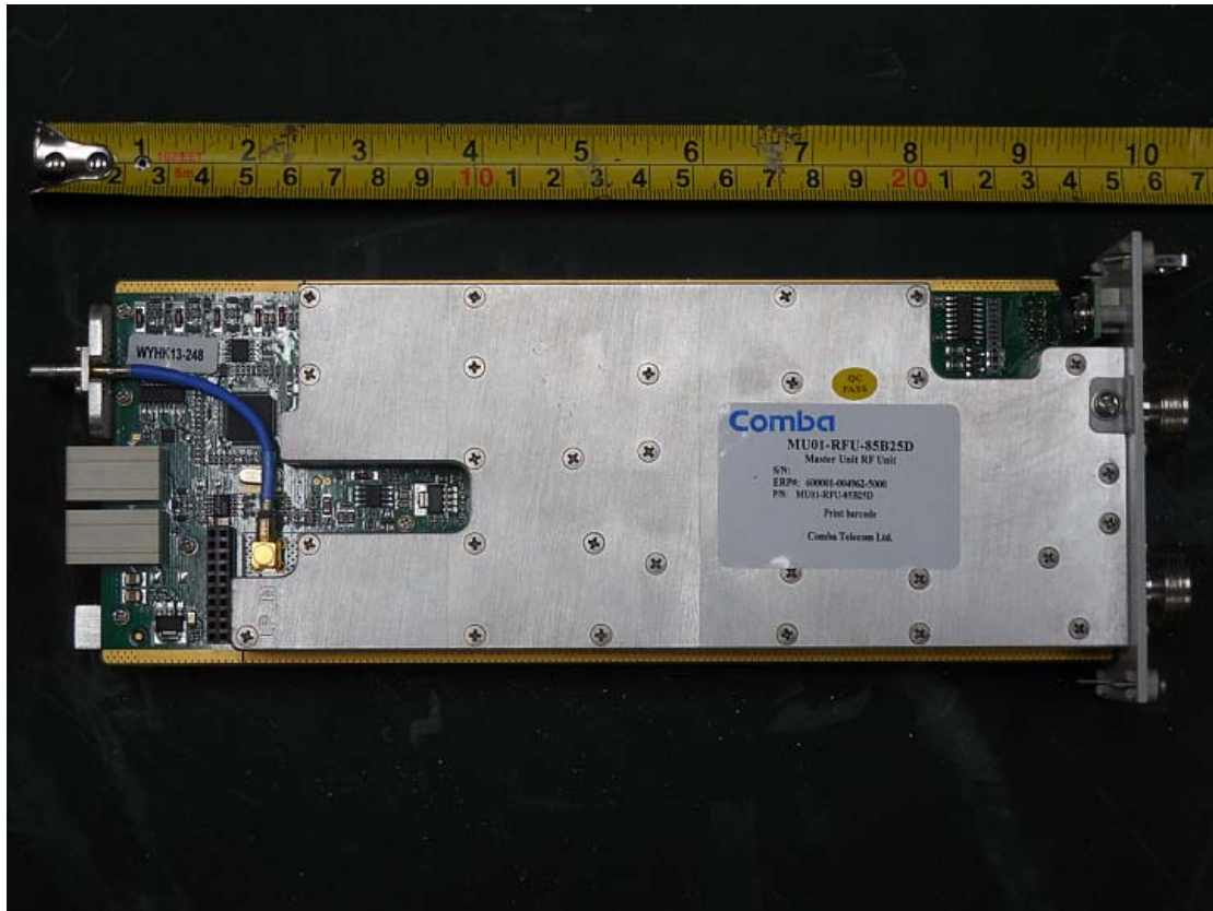
(9) MU01-RFU-85B25D
