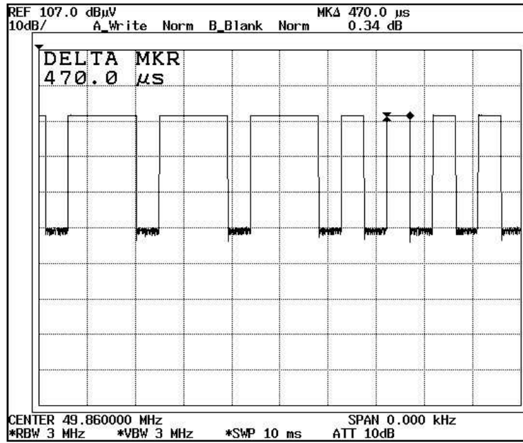
Duty Cycle 3
