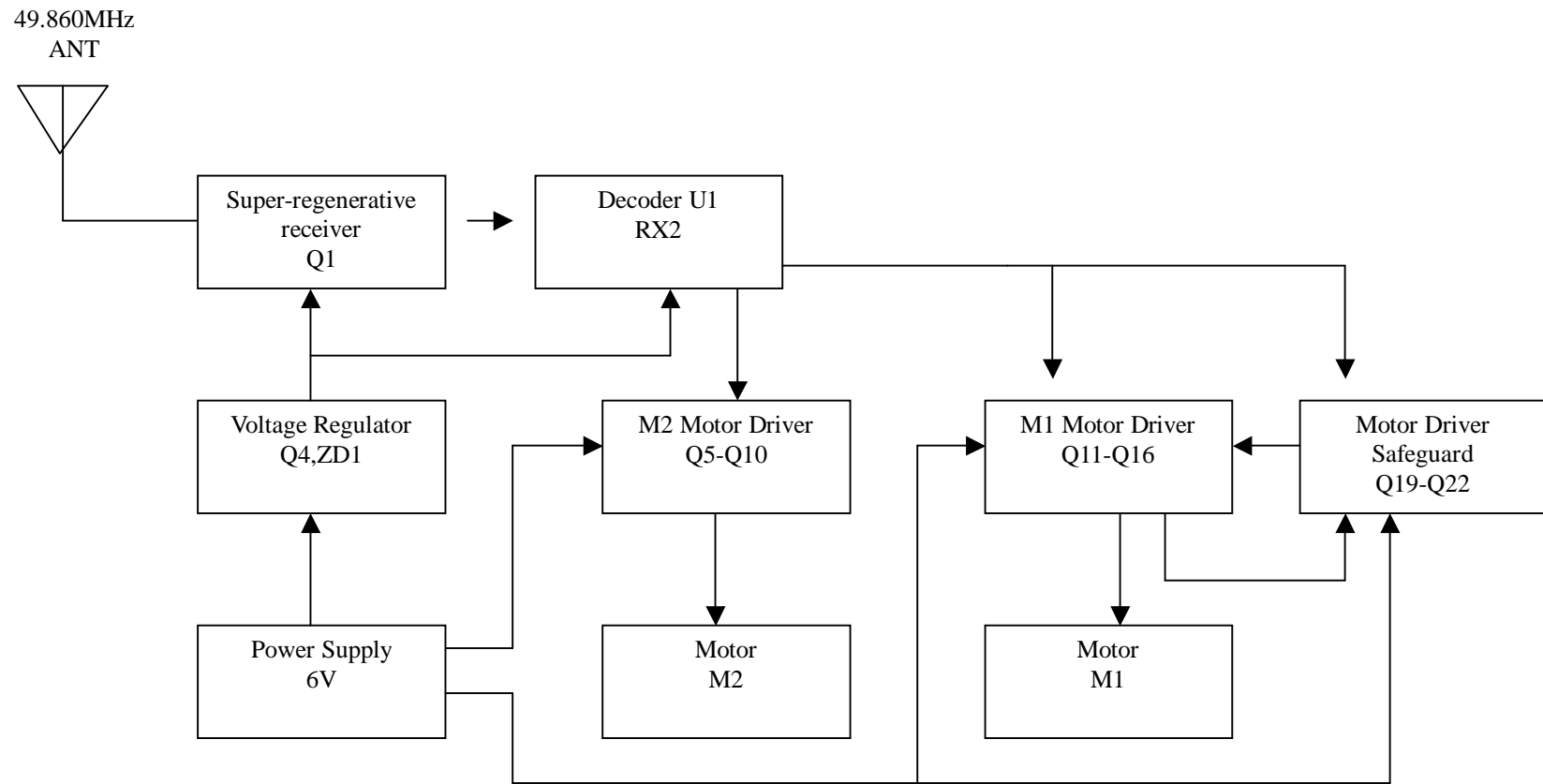
Block Diagram of RX Model: 1/10 RC CAR Jada Toys Co., Ltd.
