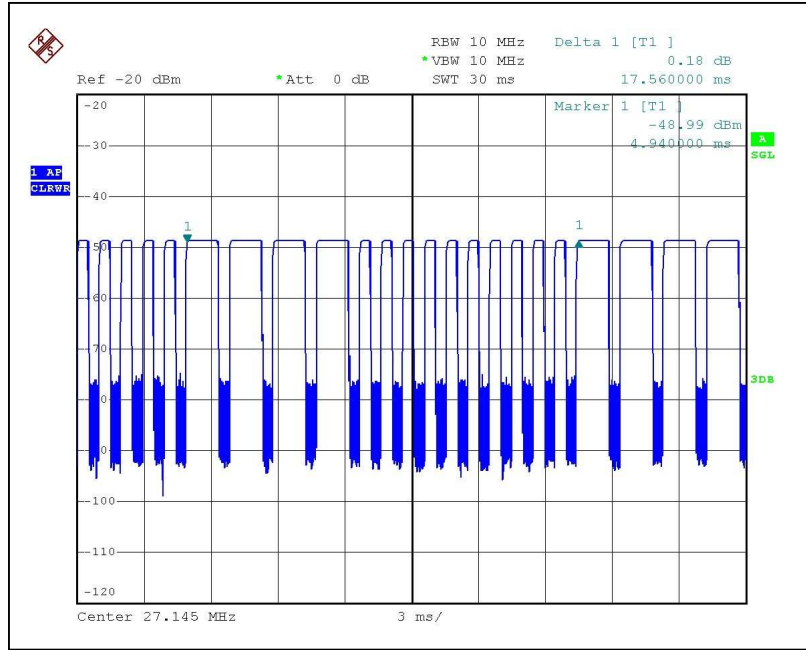
Duty Cycle 1
