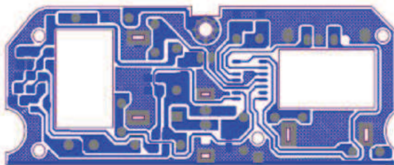
BOTTOM COPPER
