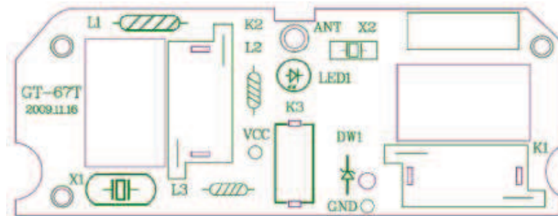
TOP SILK
