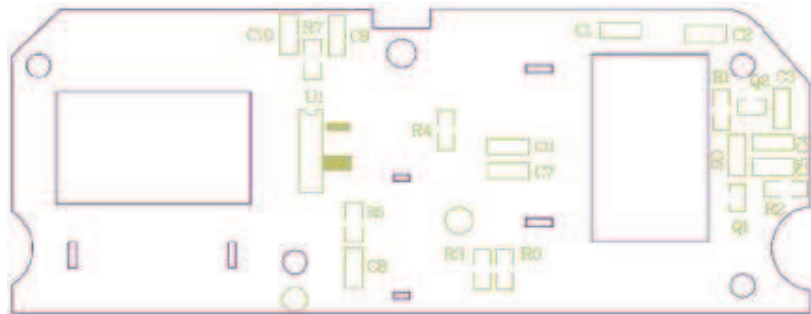
BOTTOM SILK
