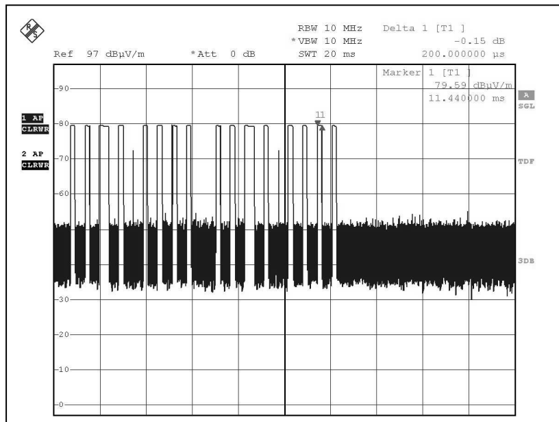
Duty Cycle 4
