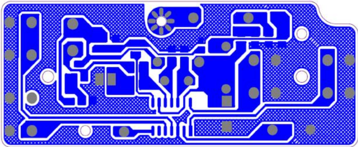
BOTTOM COPPER
