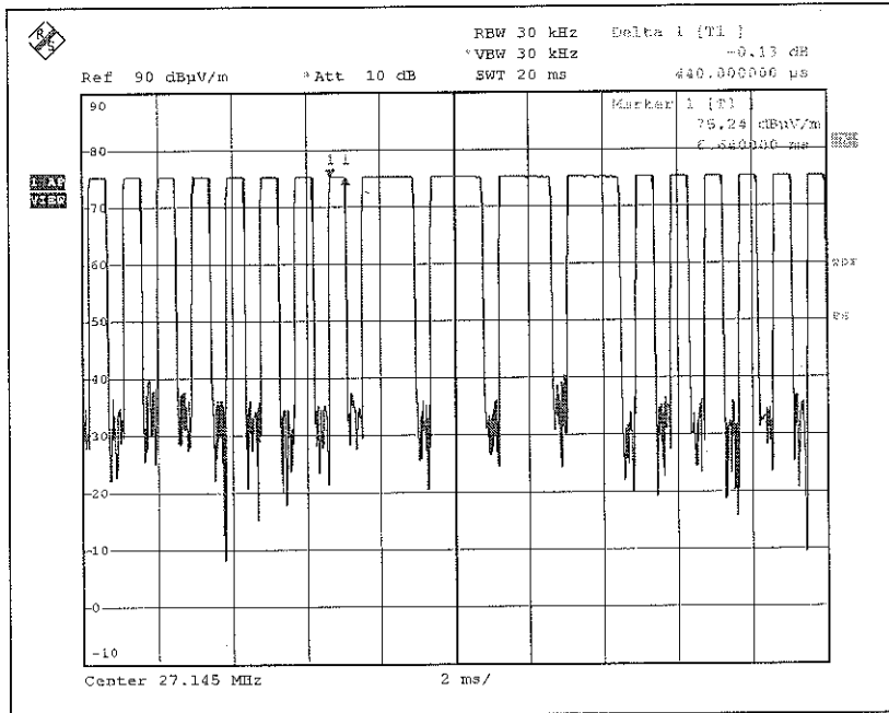
Duty Cycle 3
