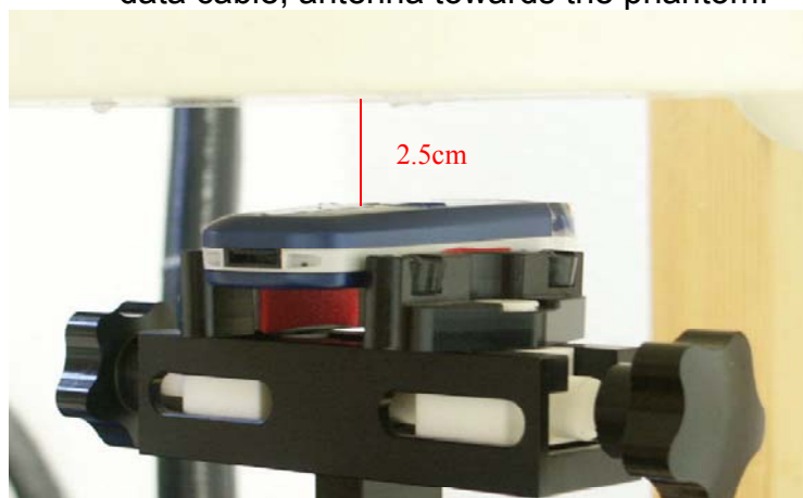
Fig. 28: Body worn configuration C65 Standard, PTT mode (Class 10), display towards the phantom.
