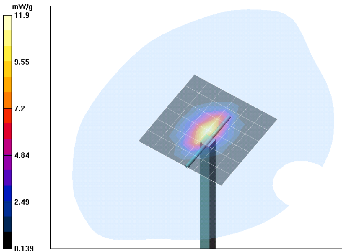
Fig. 11: Validation measurement 1900 MHz Head (December 29, 2004), coarse grid. Ambient Temperature: 21.7° C, Liquid Temperature: 21.2° C.
