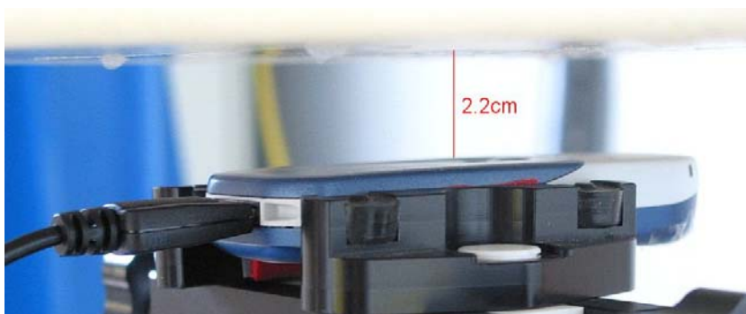
Fig. 27: Body worn configuration C65 Standard, GPRS (Class 10) with data cable, antenna towards the phantom.
