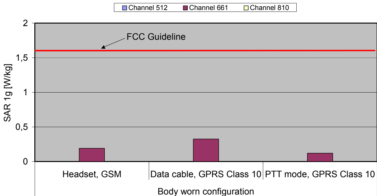
Fig. 10: The measured SAR values in body-worn configuration for the Siemens C65 with standard cover for PCS 1900 in comparison to the FCC exposure limit.
