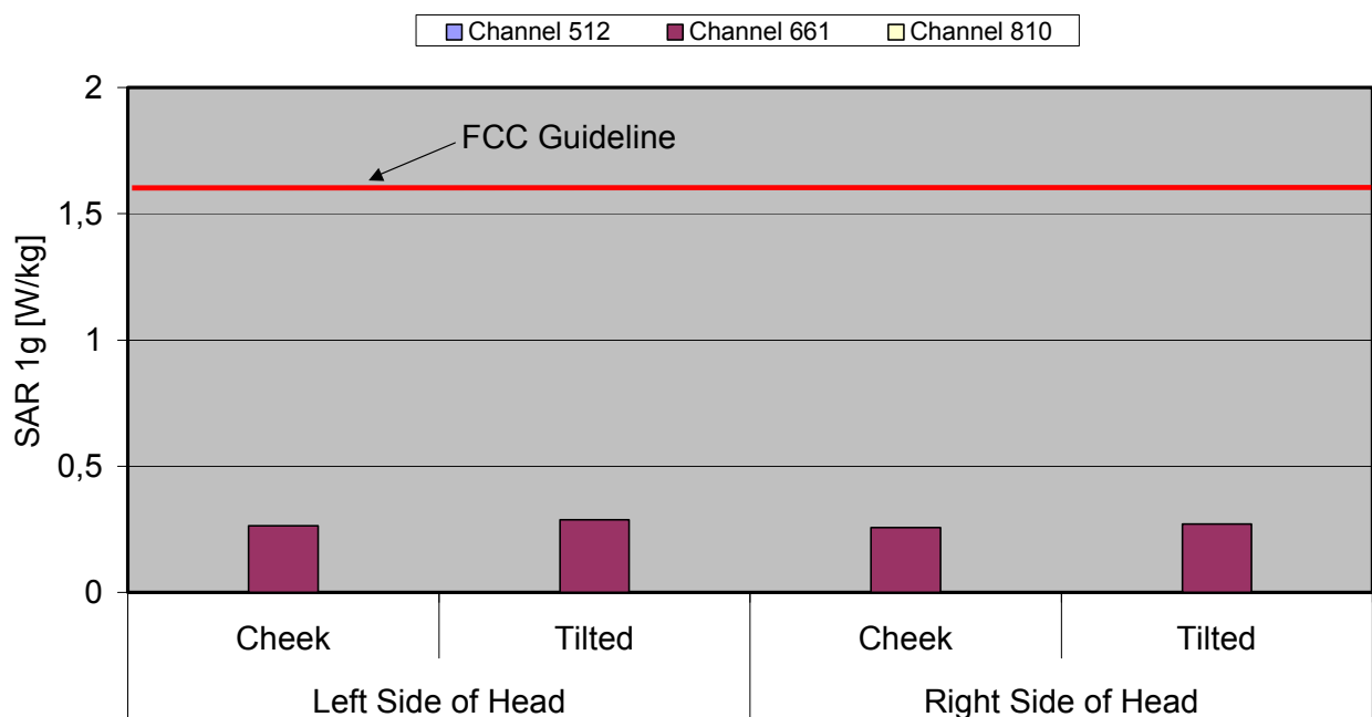
Fig. 9: The measured head phantom SAR values for the Siemens C65 with standard cover with Flash for PCS 1900 in comparison to the FCC exposure limit.
