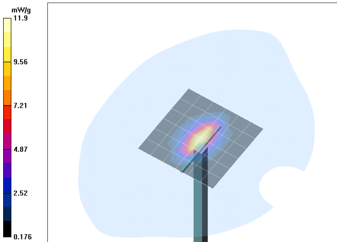
Fig. 12: Validation measurement 1900 MHz body (January 04, 2005), coarse grid. Ambient Temperature: 22.0° C, Liquid Temperature: 21.0° C.
