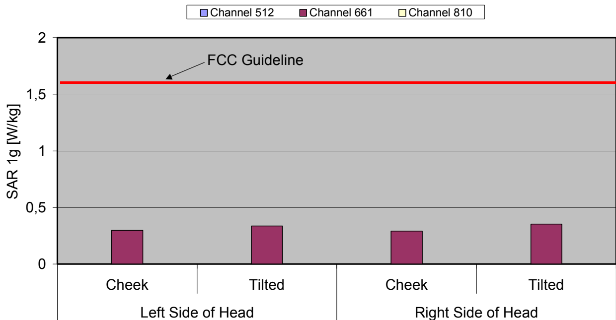
Fig. 8: The measured head phantom SAR values for the Siemens C65 with standard cover for PCS 1900 in comparison to the FCC exposure limit.
