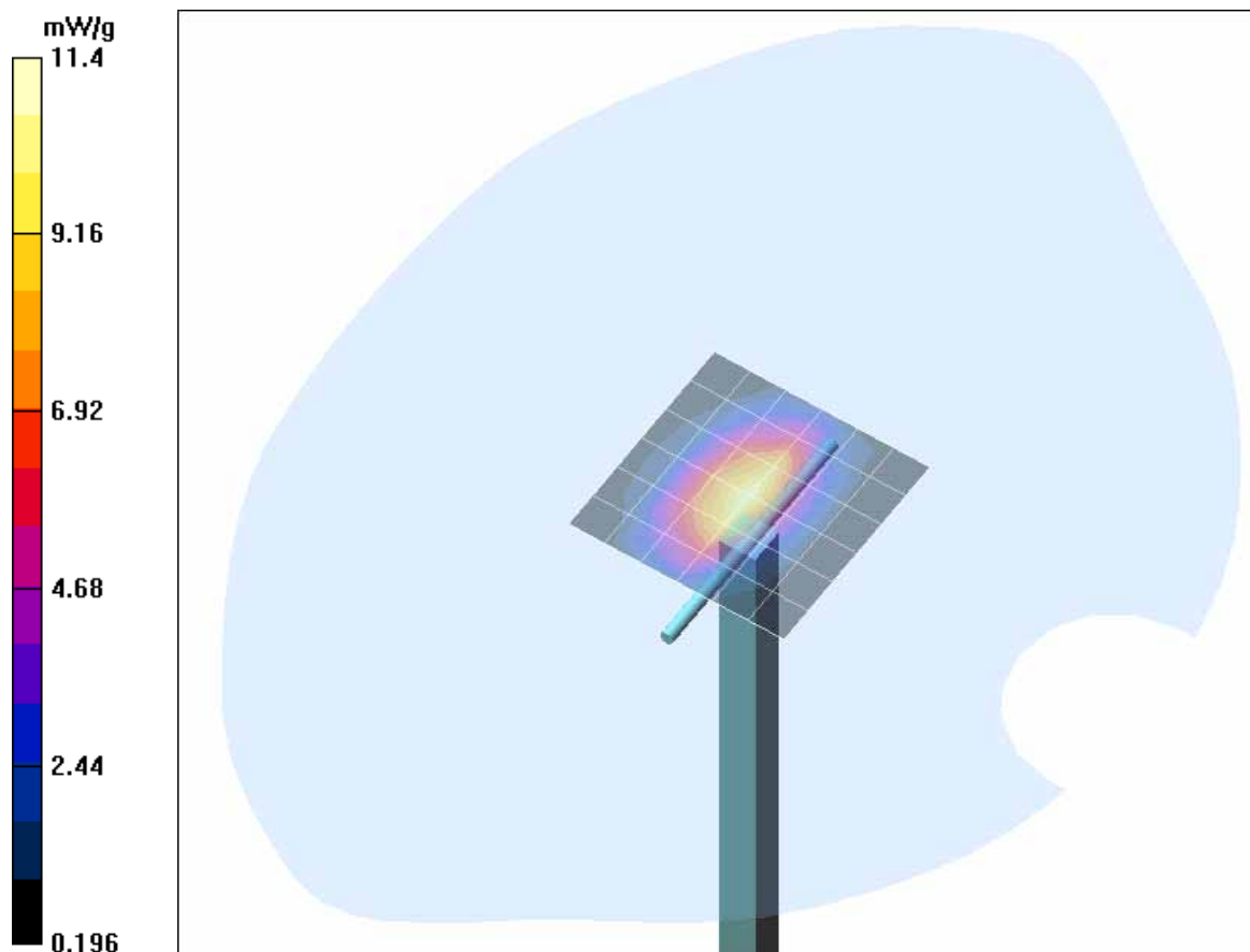
Fig. 11: Validation measurement 1900 MHz body (August 30, 2005), coarse grid. Ambient Temperature: 22.0° C, Liquid Temperature: 21.5° C.
