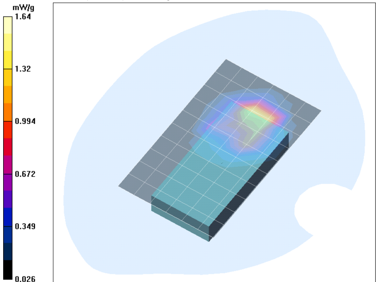
Fig. 13: SAR distribution for PCS 1900, channel 512, body worn configuration, antenna towards the phantom, with headset, with 0 mm distance (August 23, 2005; Ambient Temperature: 22.1° C; Liquid Temperature: 21.3° C).
