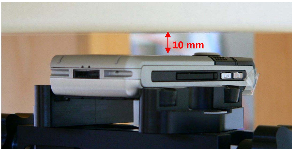
Fig. 31: Body worn configuration Siemens SXG75, GPRS (Class 10) mode without accessory and with activated bluetooth, antenna towards the phantom, gap= 10 mm.
