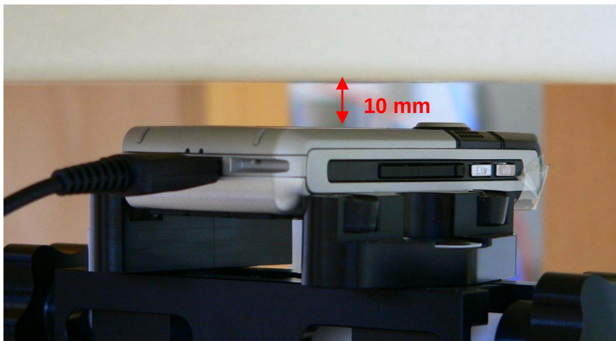
Fig. 32: Body worn configuration Siemens SXG75, GPRS (Class 10) mode with data cable, antenna towards the phantom, gap= 10 mm.
