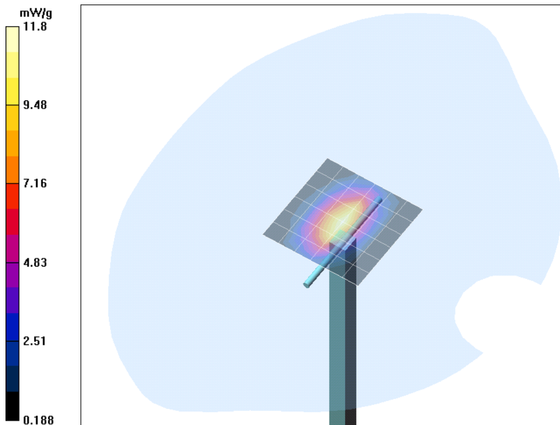
Fig. 11: Validation measurement 1900 MHz body (August 23, 2005), coarse grid. Ambient Temperature: 22.1° C, Liquid Temperature: 21.0° C.
