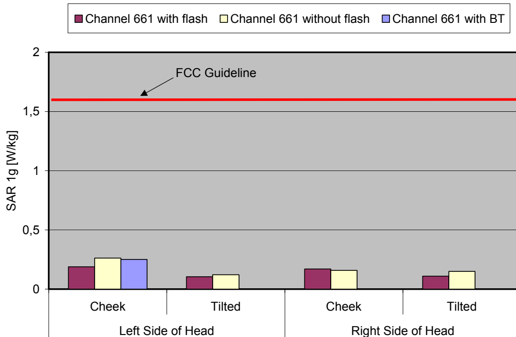
Fig. 8: The measured head phantom SAR values for the Siemens SXG75 for PCS 1900 in comparison to the FCC exposure limit.
