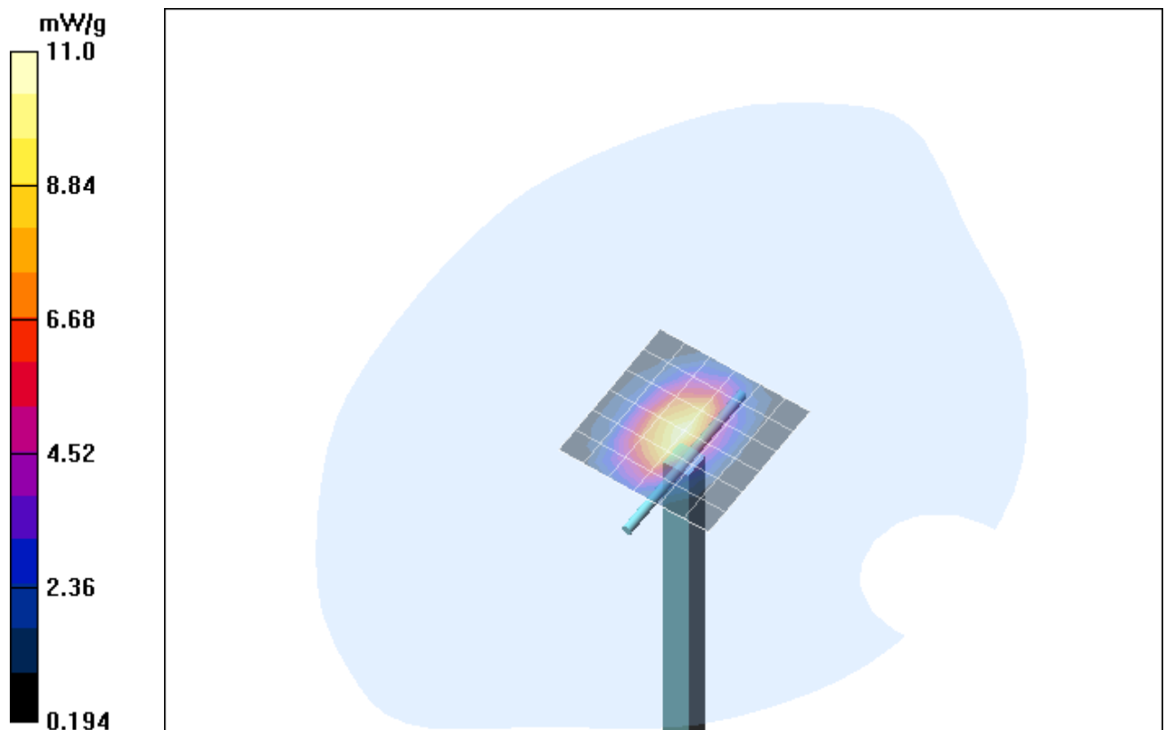
Fig. 10: Validation measurement 1900 MHz Head (August 22, 2005), coarse grid. Ambient Temperature: 22.0° C, Liquid Temperature: 21.0° C.
