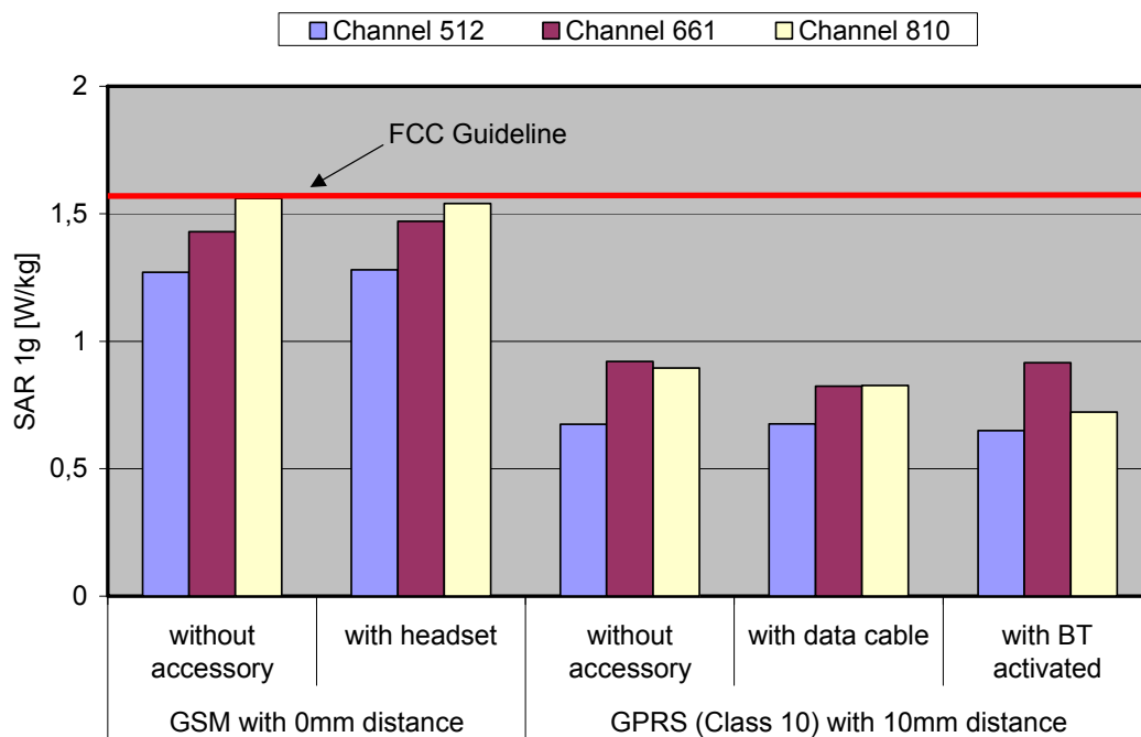
Fig. 8: The measured head phantom SAR values for the Siemens SXG75 for PCS 1900 in comparison to the FCC exposure limit.
