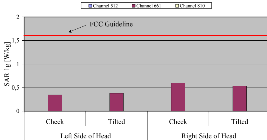
Fig. 8: The measured head phantom SAR values for the Siemens SX1 (Sample 2) for PCS 1900 in comparison to the FCC exposure limit.
