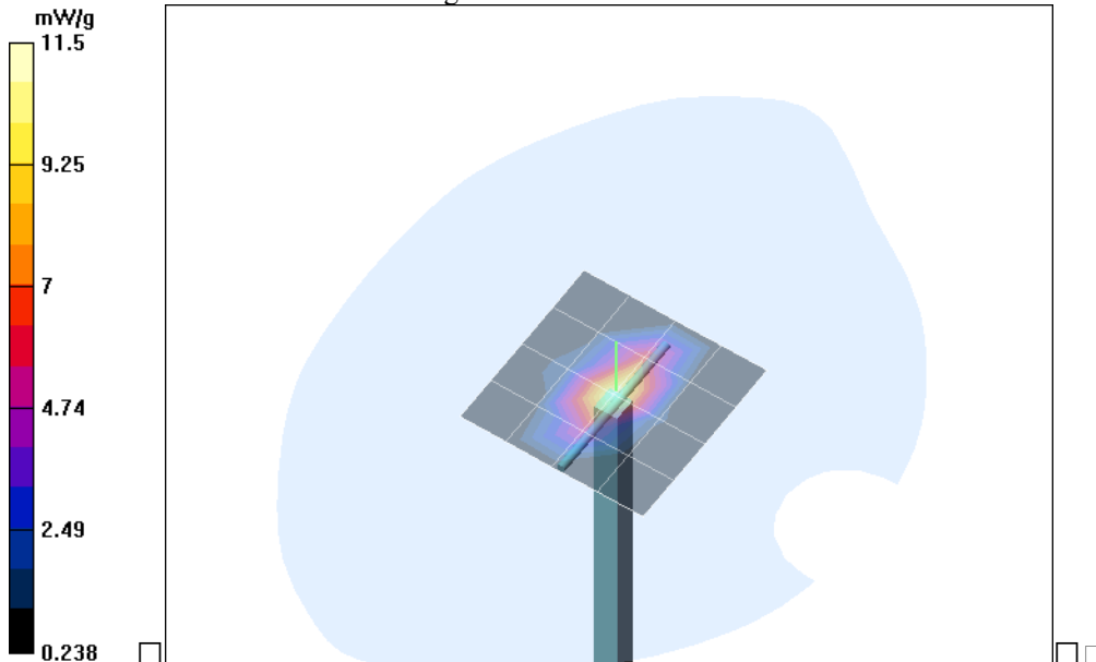
Fig. 12: Validation measurement 1900 MHz body (23.07.2003), coarse grid. Ambient Temperature: 21.3° C, Liquid Temperature: 20.3° C.
