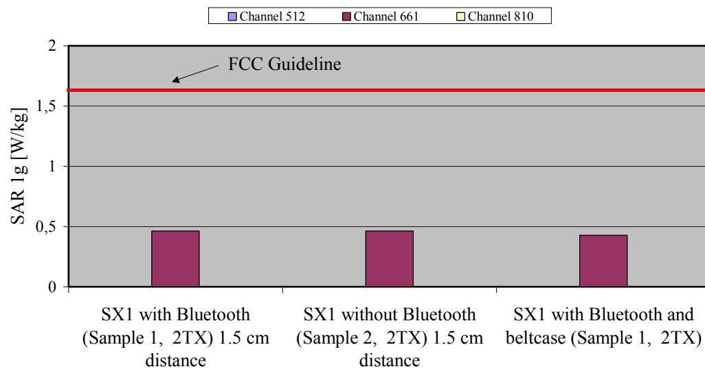
Fig. 10: The measured SAR values in body-worn configuration (GPRS mode) for the Siemens SX1 distance for PCS 1900 in comparison to the FCC exposure limit.
