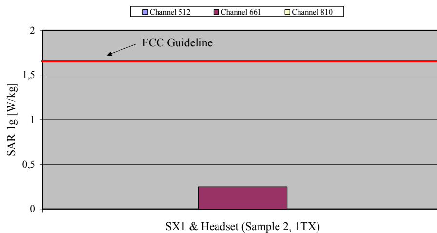
Fig. 9: The measured SAR values in body-worn configuration (GSM mode) for the Siemens SX1 with 1.5 cm distance for PCS 1900 in comparison to the FCC exposure limit.
