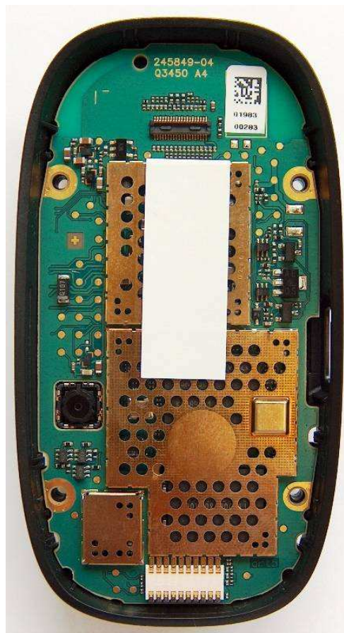
Disassemble Step 7: Rear Cover Base with PCB
