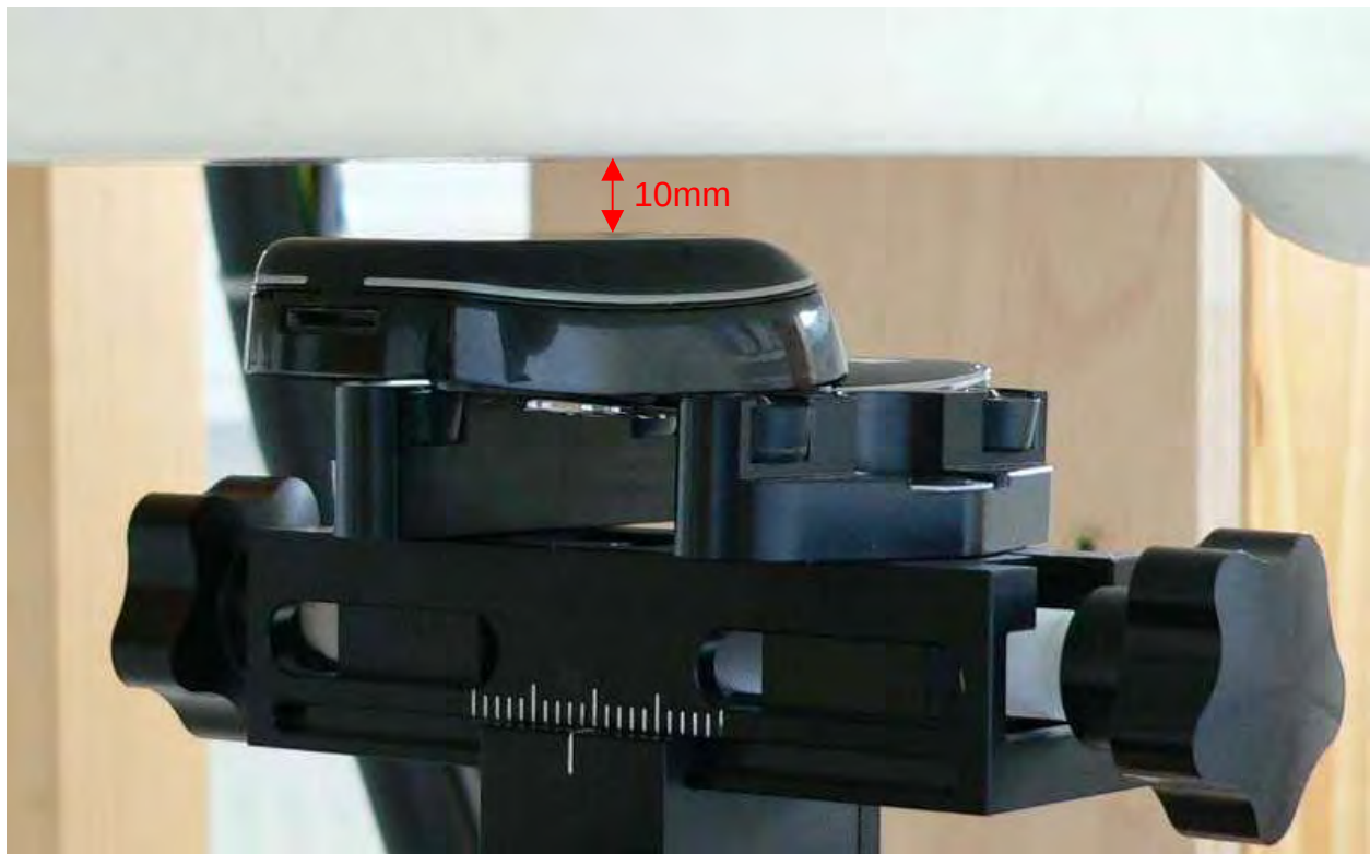
Fig. 30: Body worn configuration, GSM and GPRS (Class 10) without accessory, antenna towards the phantom, slider up.
