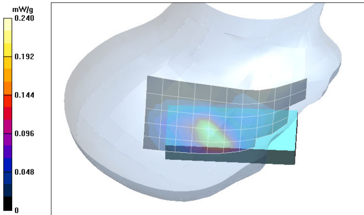
Fig. 3: SAR distribution for PCS 1900, channel 661, cheek position, right side of head. (03.06.2004; Ambient Temperature: 21.1° C; Liquid Temperature : 20.0° C).
