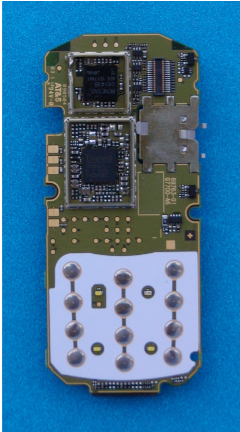
SL65 PCB Rear View Shields Removed
