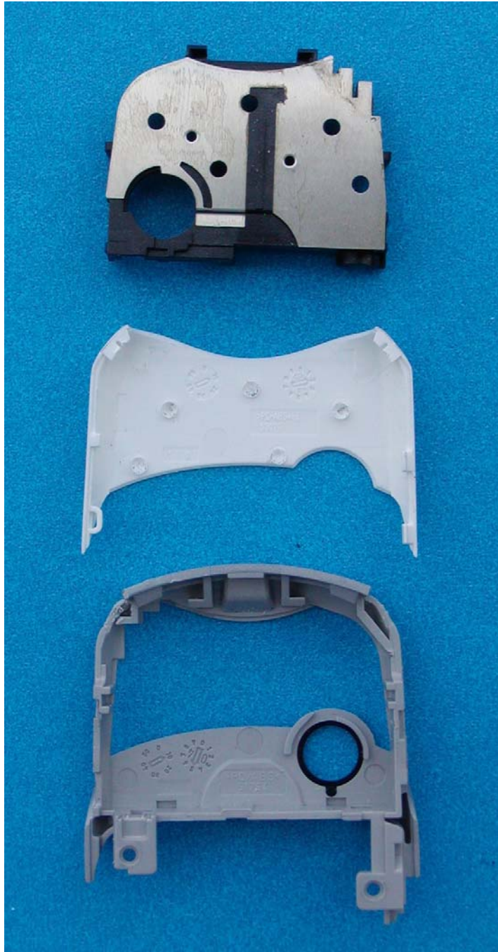
SL65 Disassembly step 3
