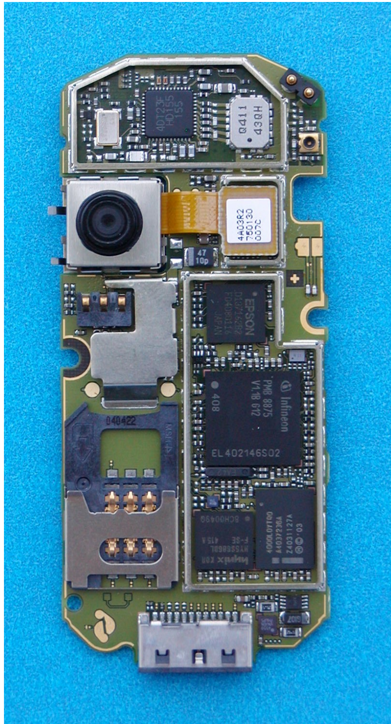
SL65 PCB Front View Shields Removed
