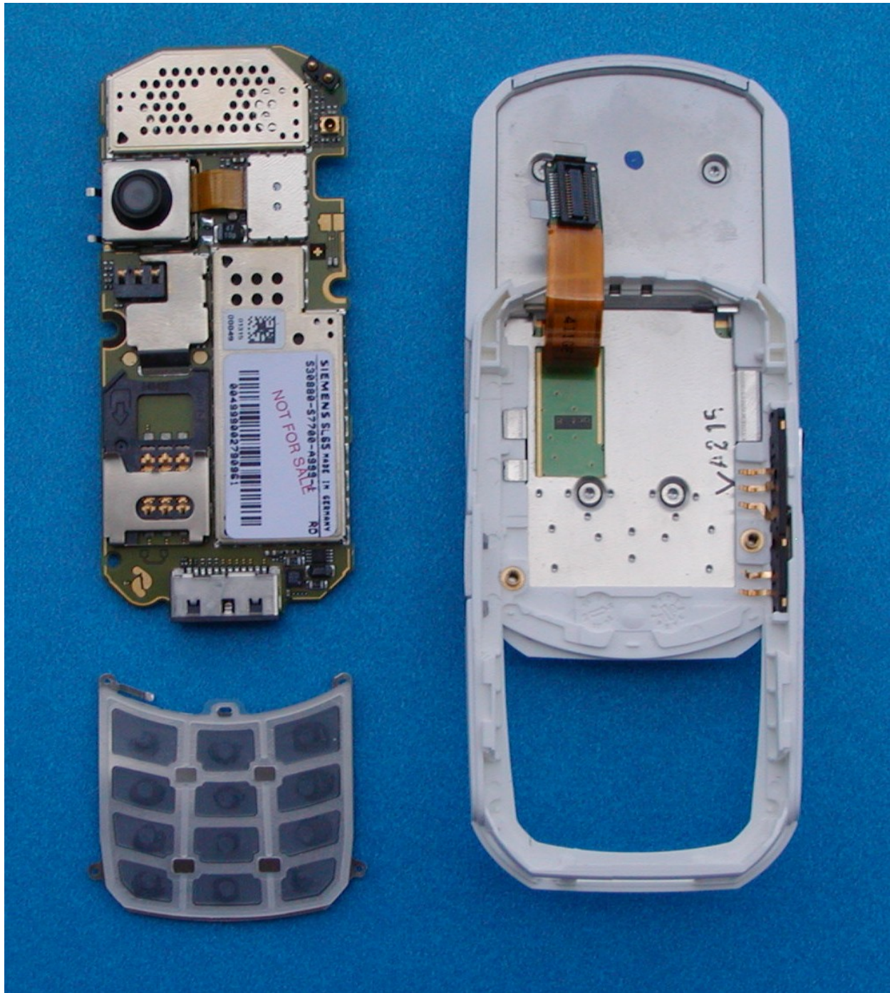
SL65 Disassembly step 2
