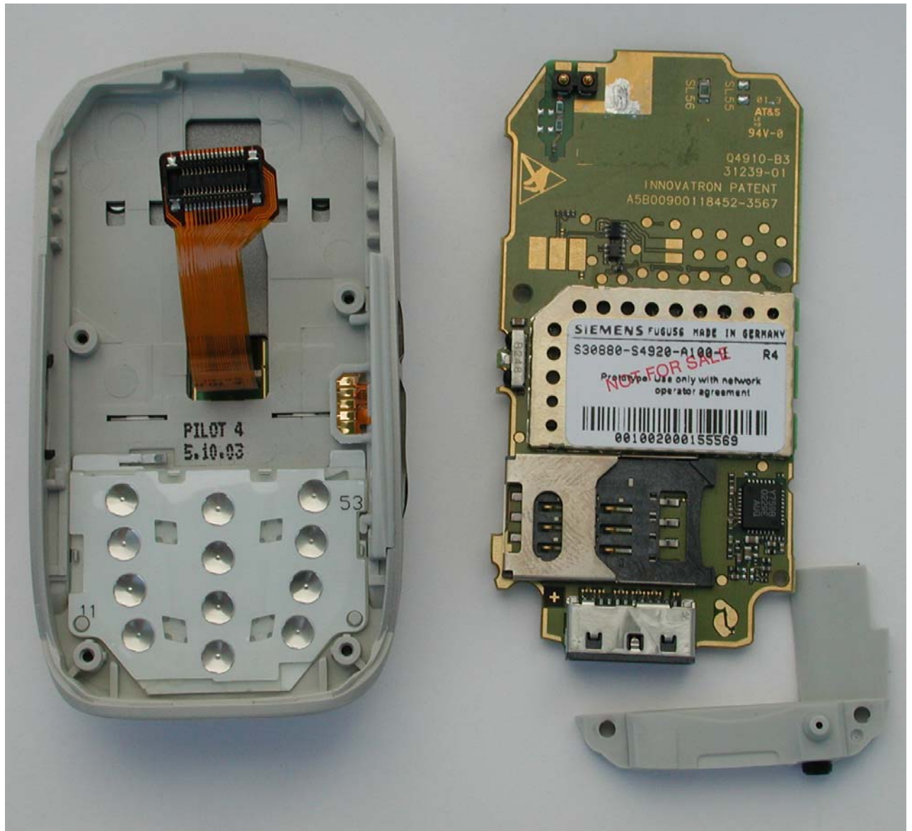
SL56 Disassembly step 2
