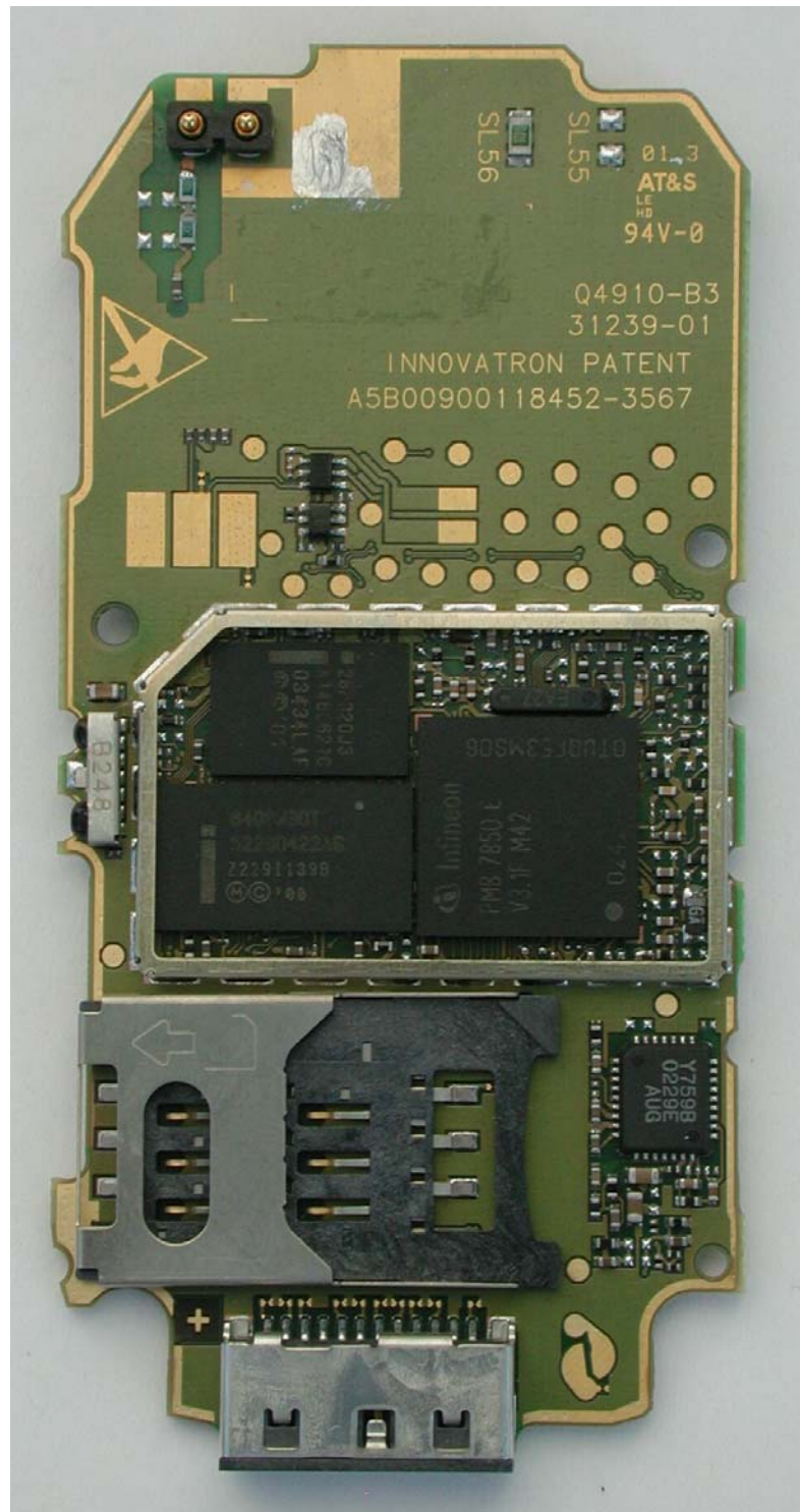
SL56 board without shielding, side2
