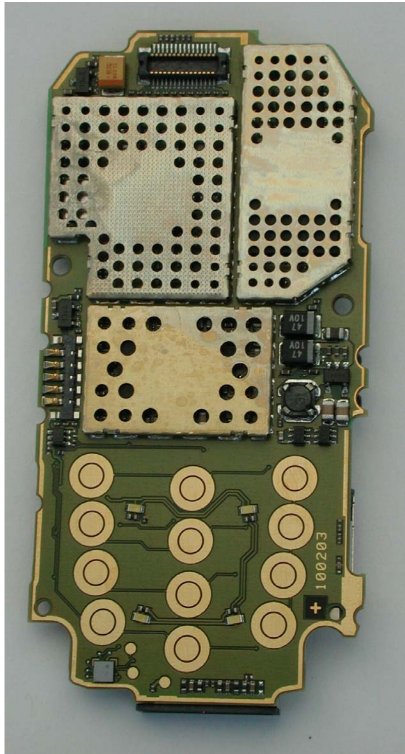
SL56 board with shielding, side1
