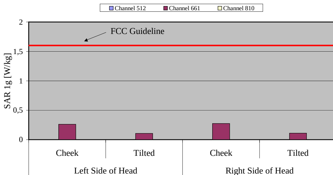
Fig. 11: The measured head phantom SAR values for the Siemens SL55, slider up, with camera for PCS 1900 in comparison to the FCC exposure limit.
