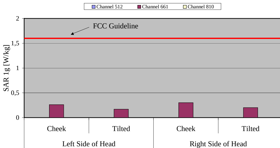
Fig. 12: The measured head phantom SAR values for the Siemens SL55, slider down, with camera for PCS 1900 in comparison to the FCC exposure limit.
