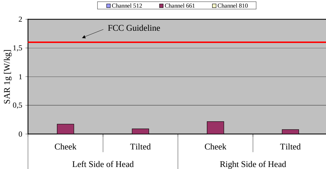
Fig. 9: The measured head phantom SAR values for the Siemens SL55, slider up, without camera for PCS 1900 in comparison to the FCC exposure limit.
