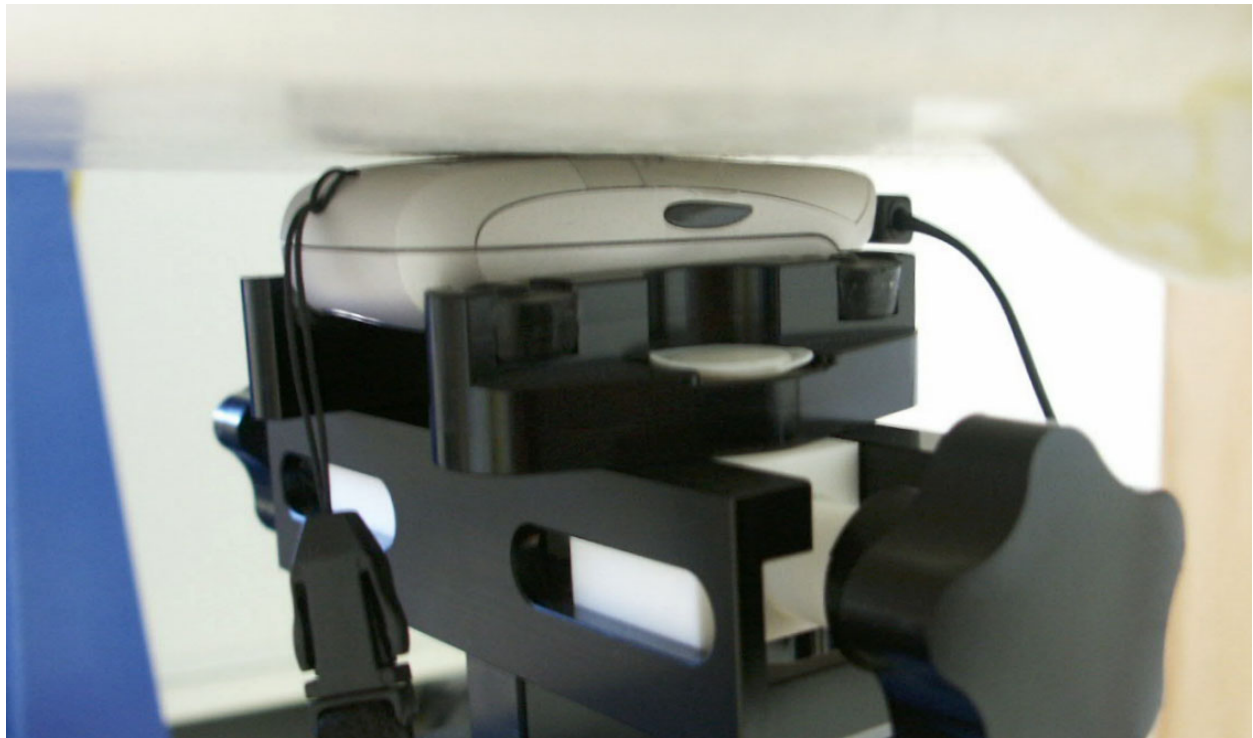
Fig. 44: Body worn configuration, slider down with headset, display towards the ground.
