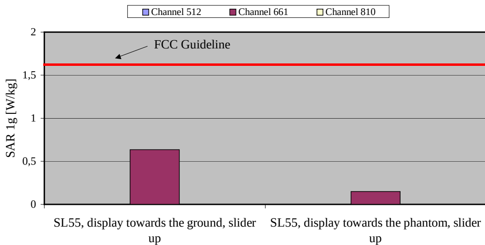
Fig. 13: The measured SAR values in body-worn configuration for the Siemens SL55, slider up, with headset for PCS 1900 in comparison to the FCC exposure limit.
