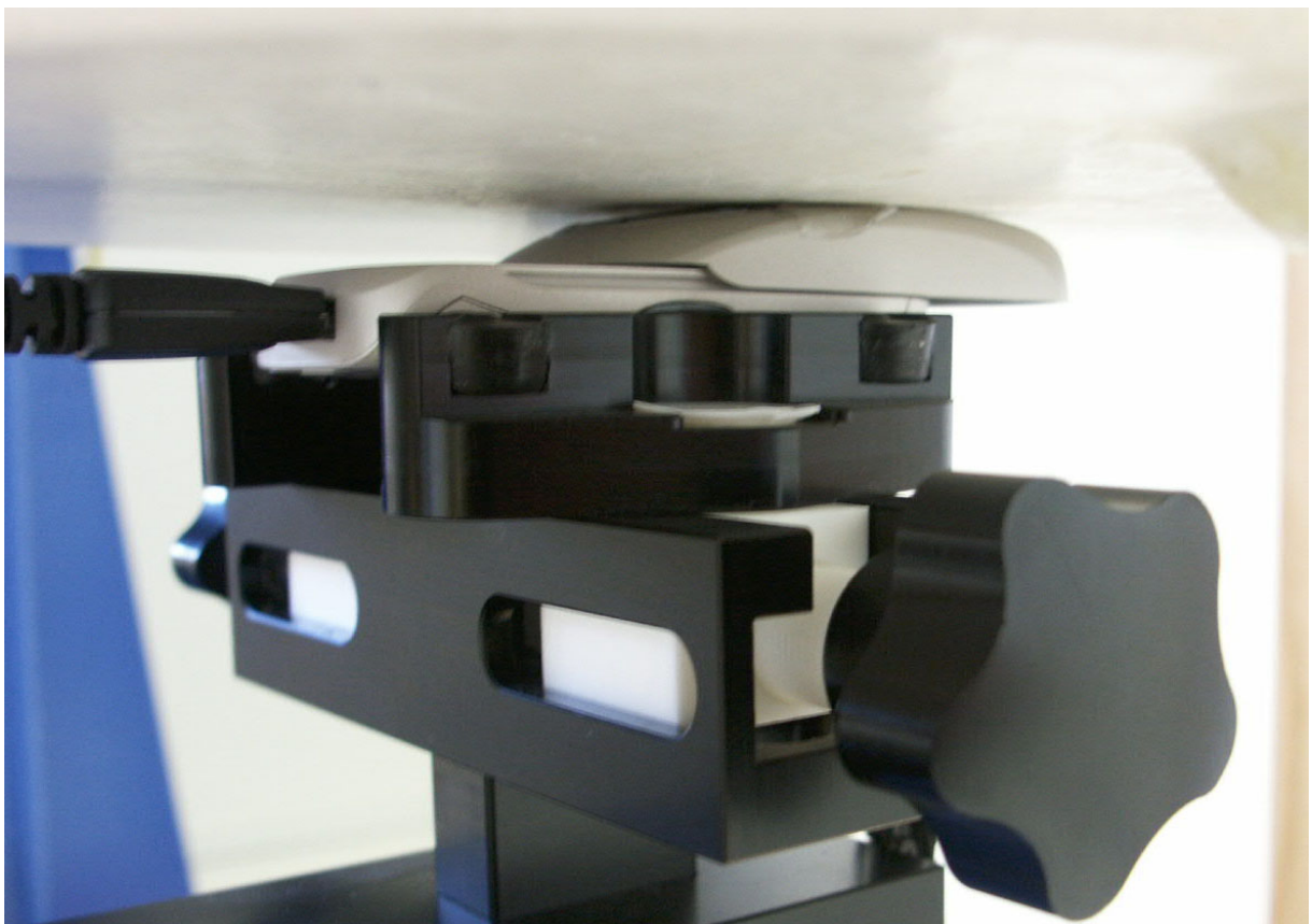
Fig. 47: Body worn configuration, slider up with data cable, display towards the phantom.
