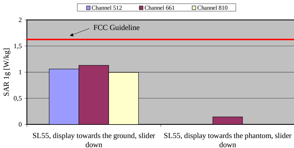
Fig. 14: The measured SAR values in body-worn configuration for the Siemens SL55, slider down, with headset for PCS 1900 in comparison to the FCC exposure limit.
