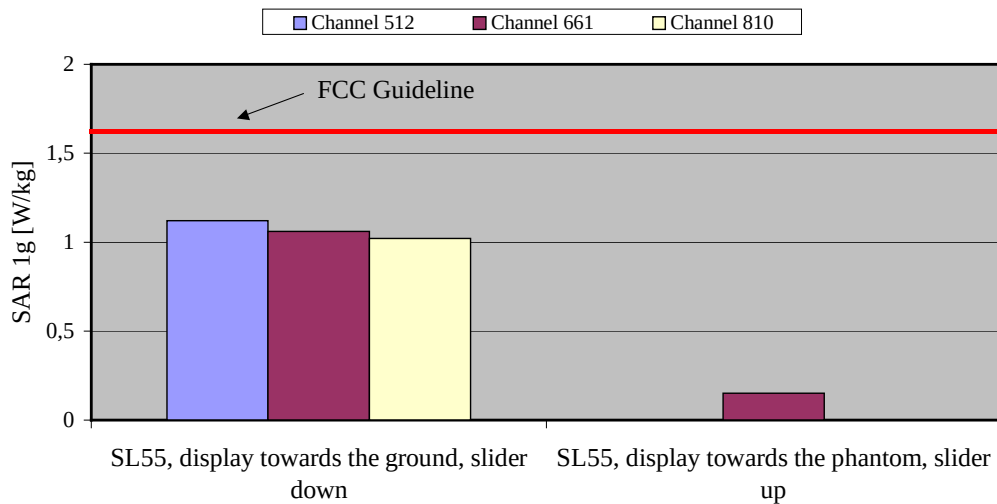
Fig. 15: The measured worst case SAR values in body-worn configuration for the Siemens SL55, with data cable (GPRS mode, 1 TX slot) for PCS 1900 in comparison to the FCC exposure limit.
