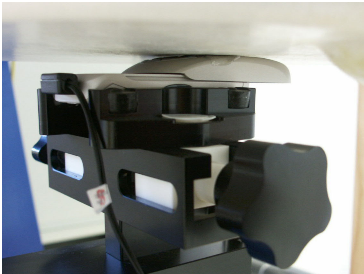
Fig. 43: Body worn configuration, slider up with headset, display towards the phantom.
