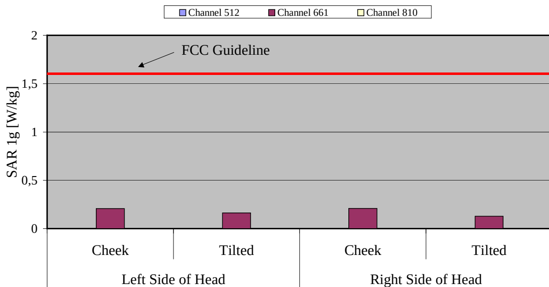
Fig. 10: The measured head phantom SAR values for the Siemens SL55, slider down, without camera, for PCS 1900 in comparison to the FCC exposure limit.
