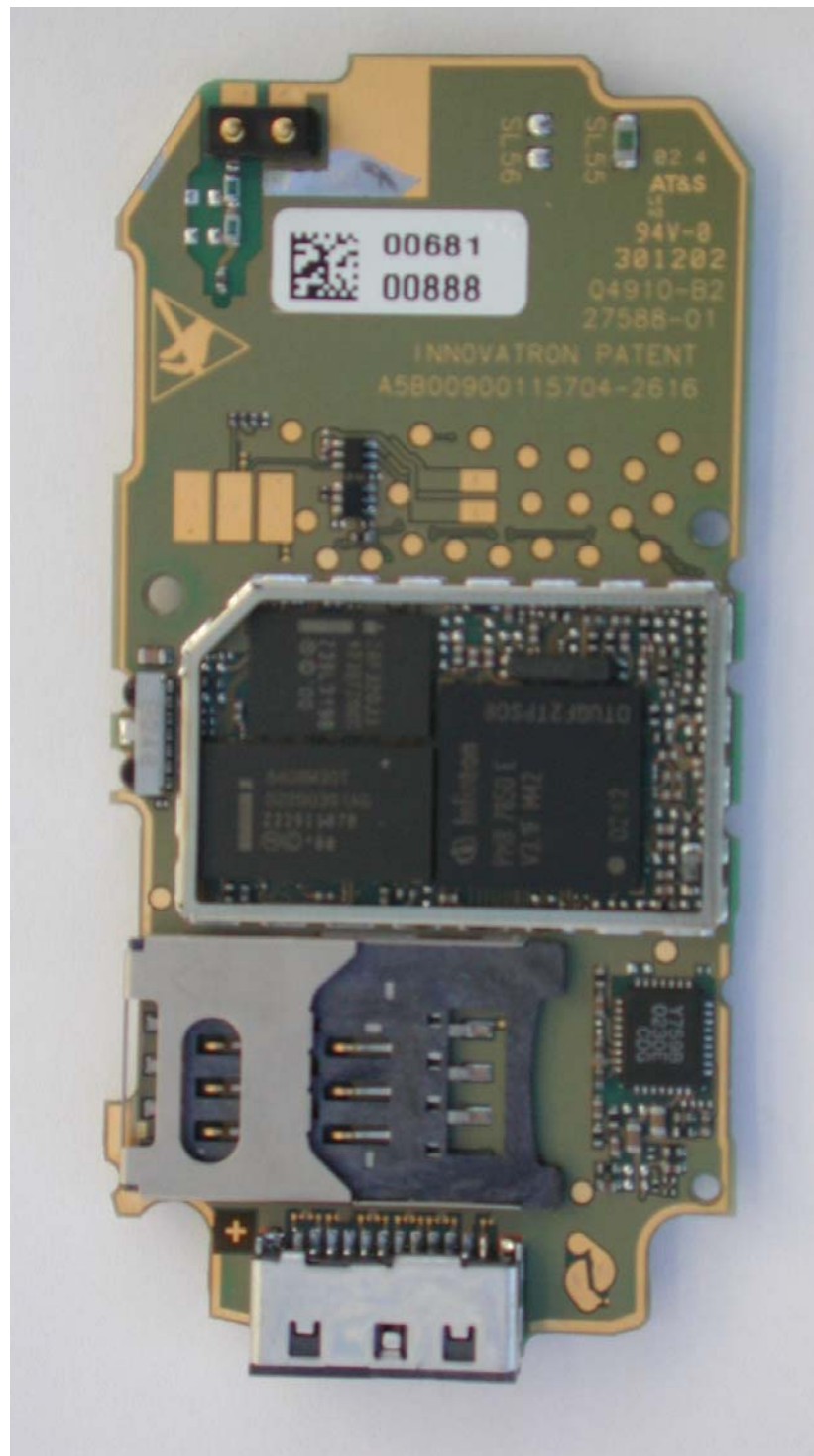
SL55 board without shielding, side2
