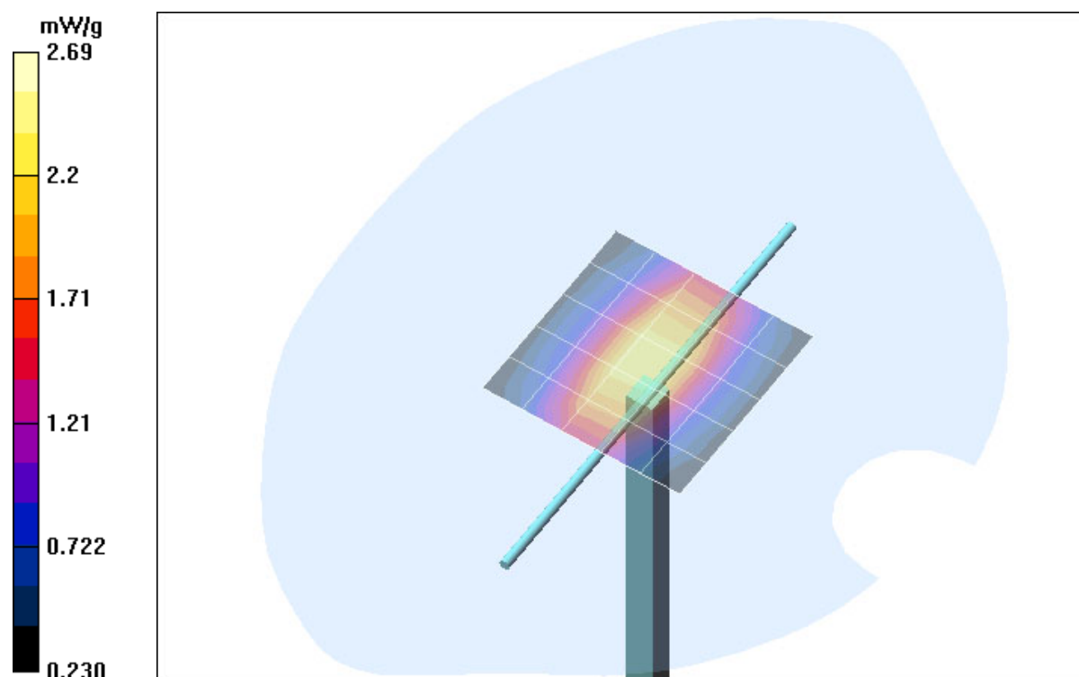
Fig. 14: Validation measurement 835MHz Head (August 18, 2004), coarse grid. Ambient Temperature: 21.9° C, Liquid Temperature: 21.3° C.
