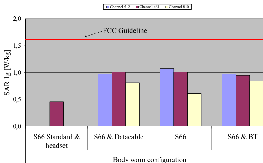
Fig. 13: The measured SAR values in body-worn configuration for the Siemens S66 for PCS 1900 (1 TX slot with headset, and 2 TX slots with and without data cable and Bluetooth, gap = 22 mm) in comparison to the FCC exposure limit.
