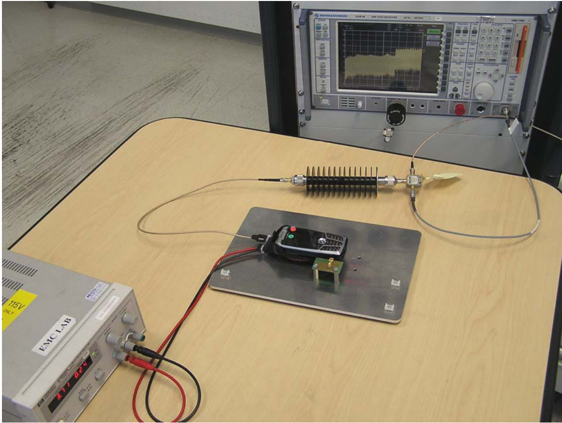
Test setup – Conducted measurements GSM
