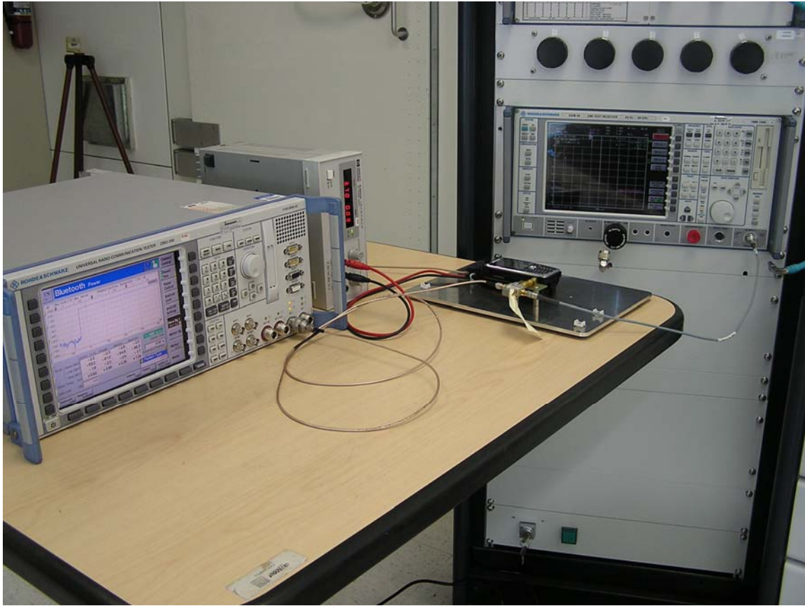
Test setup – Conducted measurements BT
