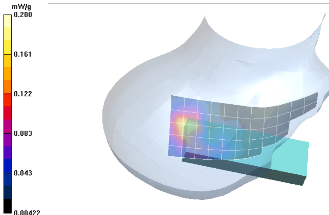
Fig. 8: SAR distribution for PCS 1900, channel 661, tilted position, right side of head. (03.05.2004; Ambient Temperature: 20.6° C; Liquid Temperature 19.4° C).
