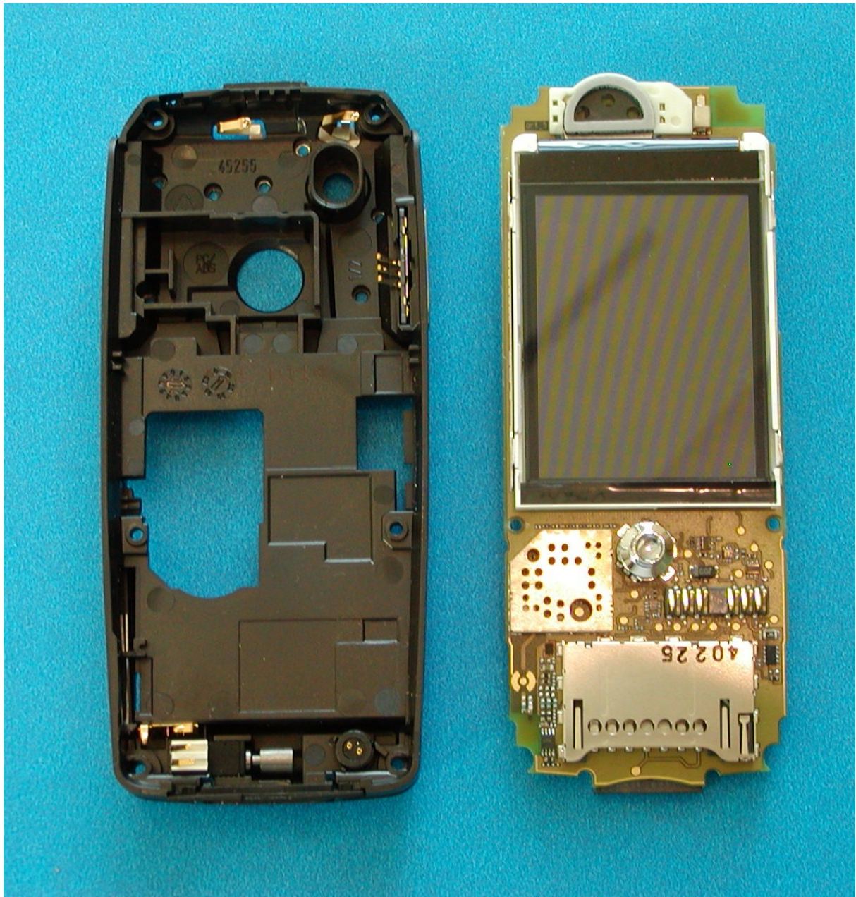
S65 Disassembly step 3
