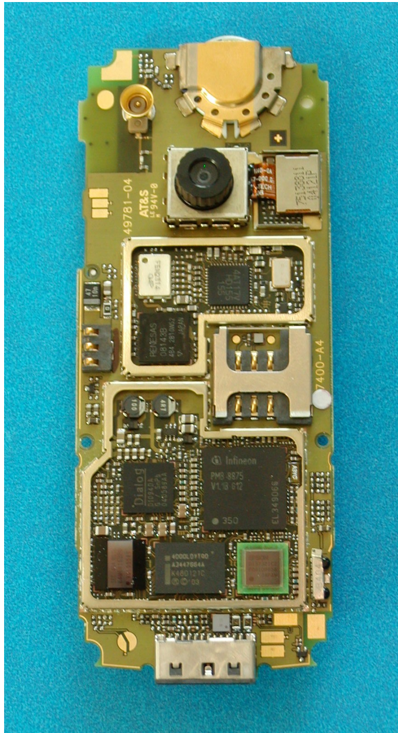
S65 PCB Rear View Shields Removed
