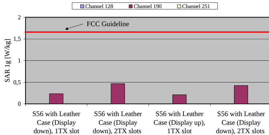
Fig. 13: The measured SAR values in body-worn configuration with Leather Case (without Headset) for the Siemens S56 for GSM 850 in comparison to the FCC exposure limit.
