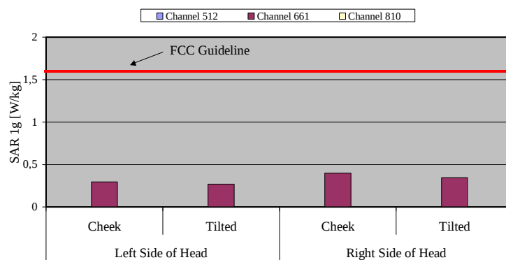
Fig. 9: The measured head phantom SAR values for the Siemens S56 for PCS 1900 in comparison to the FCC exposure limit.
