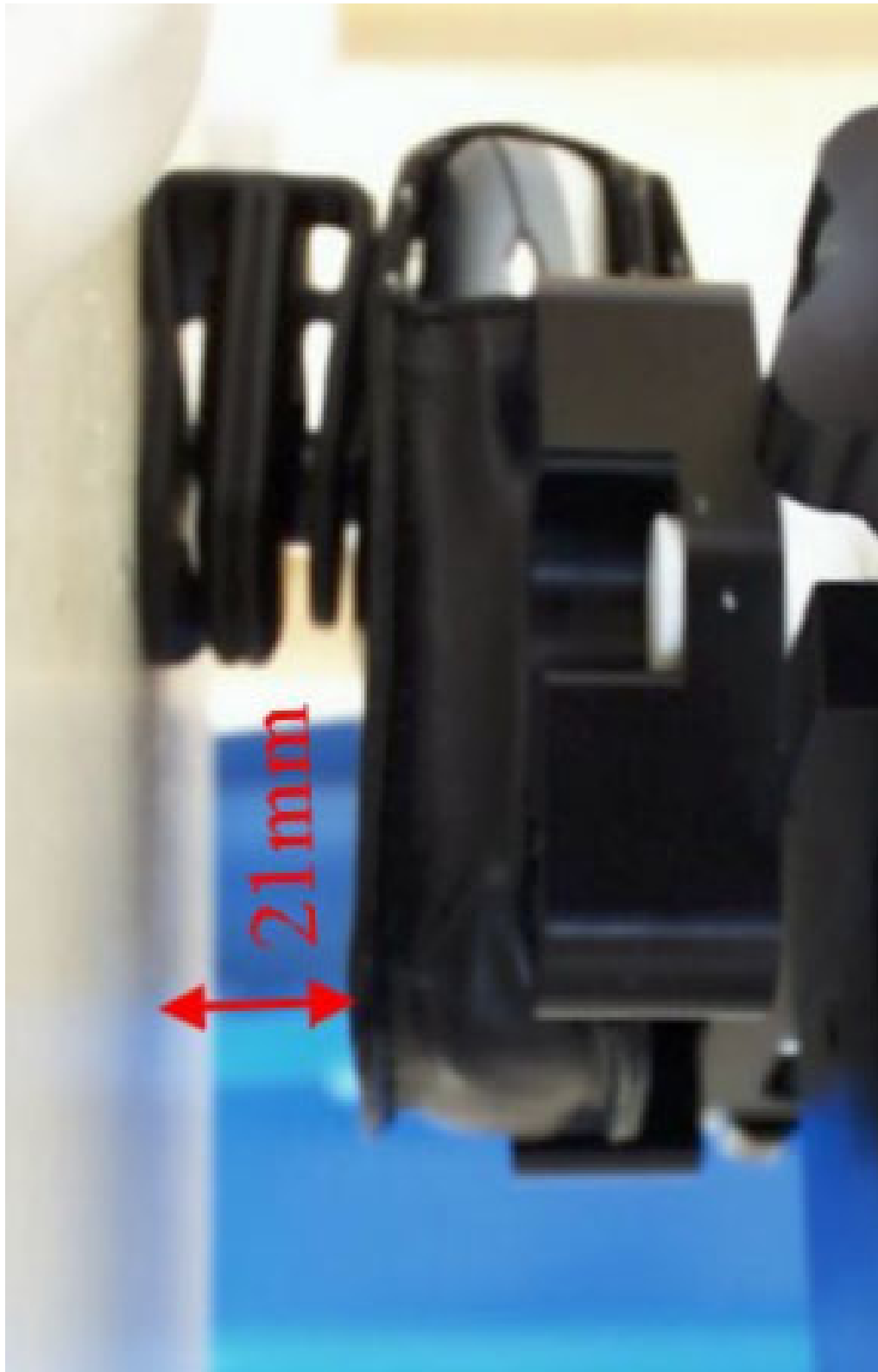
Fig. 46: Body worn configuration, Leather Case without Headset, (1 TX slot / 2 TX slots), Display down.
