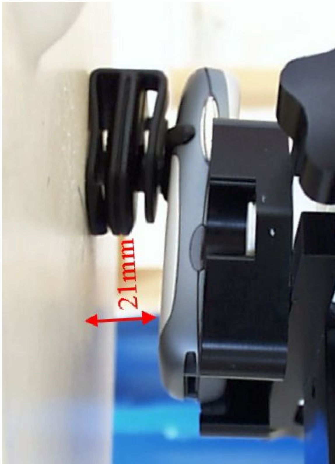
Fig. 43: Body worn configuration, Belt Clip without Headset, (1 TX slot / 2 TX slots).
