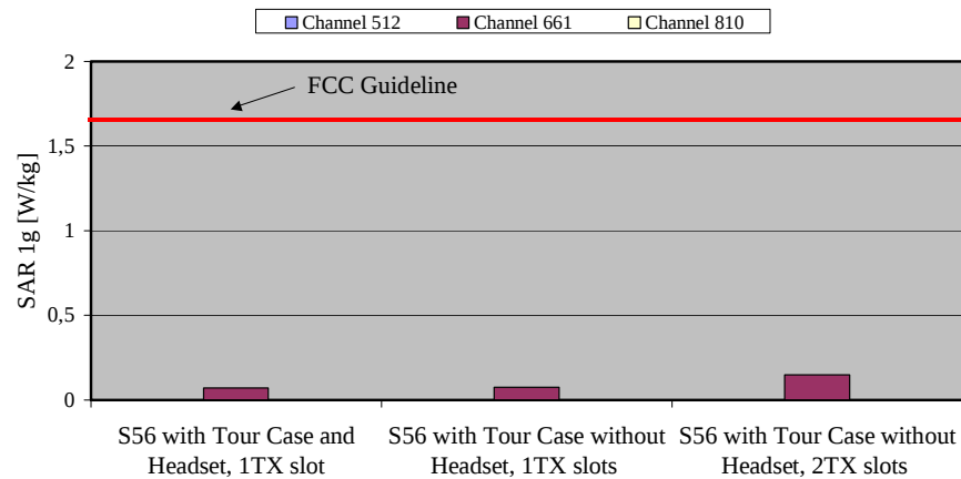
Fig. 16: The measured SAR values in body-worn configuration with Tour Case (display up) for the Siemens S56 for PCS 1900 in comparison to the FCC exposure limit.
