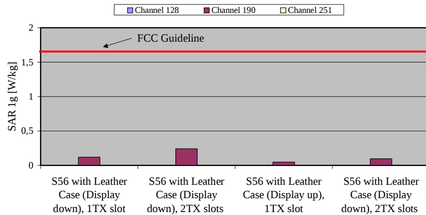
Fig. 17: The measured SAR values in body-worn configuration with Leather Case (without Headset) for the Siemens S56 for PCS 1900 in comparison to the FCC exposure limit.
