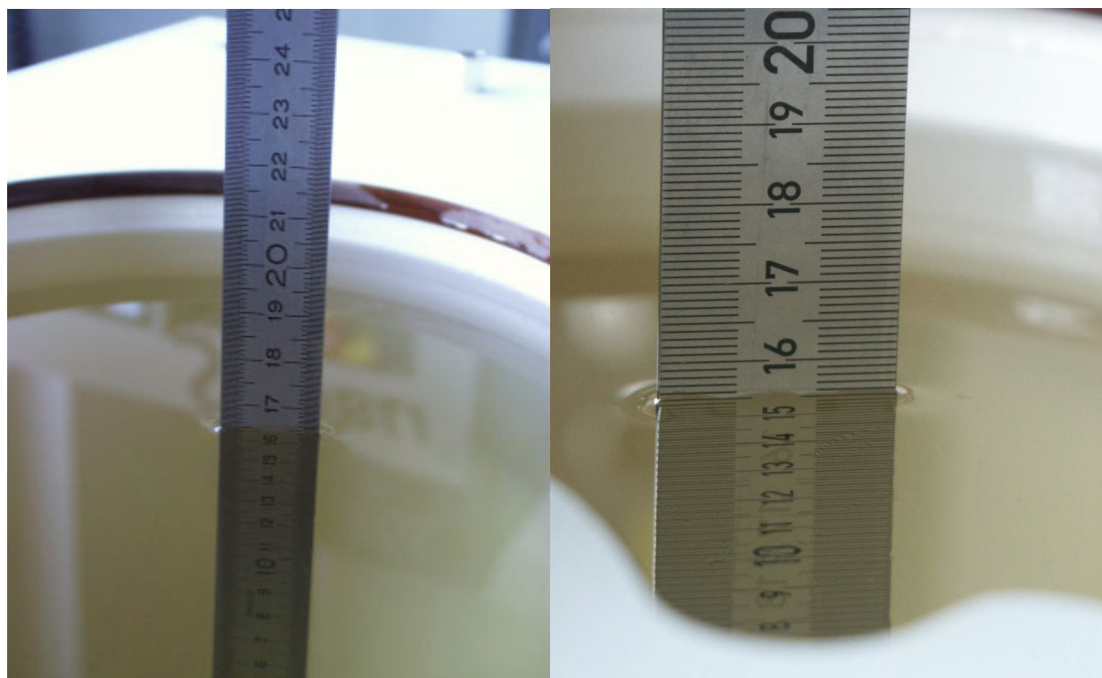
Fig. 48: Liquid depth for GSM 850 Head and Body measurements.
