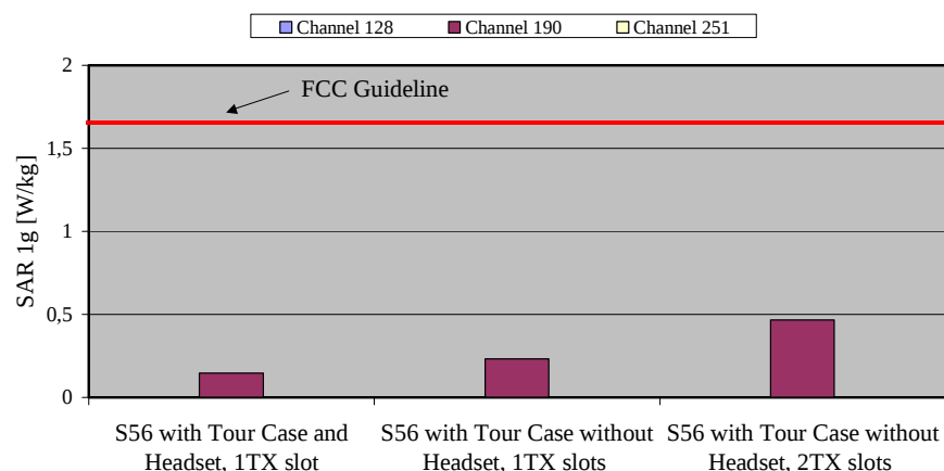
Fig. 12: The measured SAR values in body-worn configuration with Tour Case (display up) for the Siemens S56 for GSM 850 in comparison to the FCC exposure limit.
