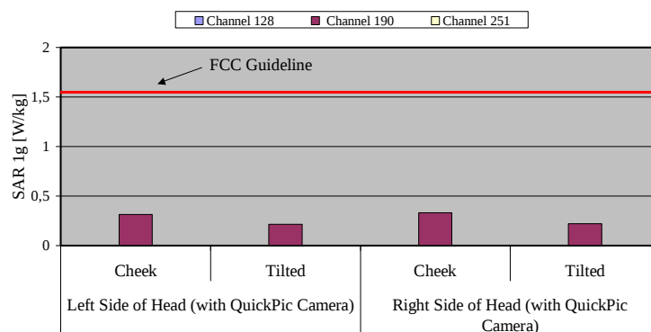
Fig. 8: The measured head phantom SAR values for the Siemens S56 with QuickPic Camera for GSM 850 in comparison to the FCC exposure limit.
