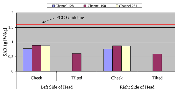
Fig. 7: The measured head phantom SAR values for the Siemens S56 for GSM 850 in comparison to the FCC exposure limit.
