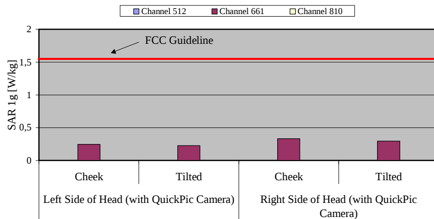
Fig. 10: The measured head phantom SAR values for the Siemens S56 with QuickPic Camera for PCS 1900 in comparison to the FCC exposure limit.
