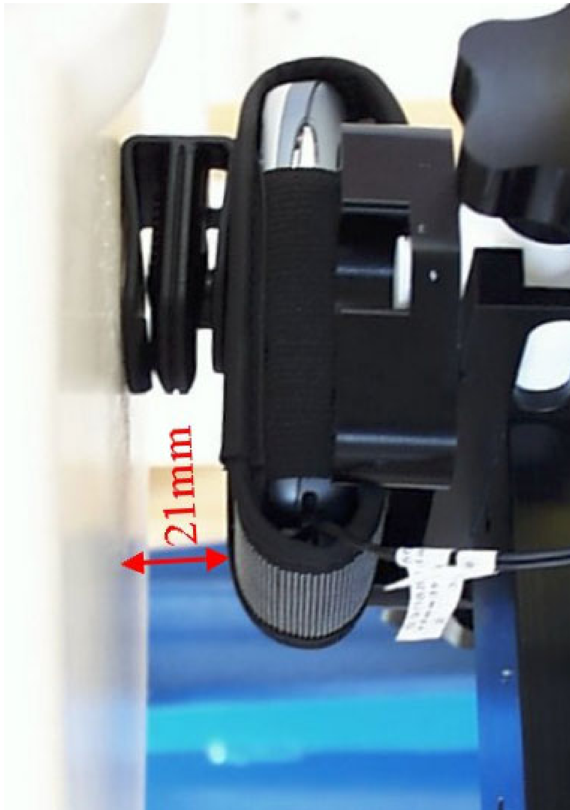
Fig. 44: Body worn configuration, Tour Case with Headset (1 TX slot), Display up.
