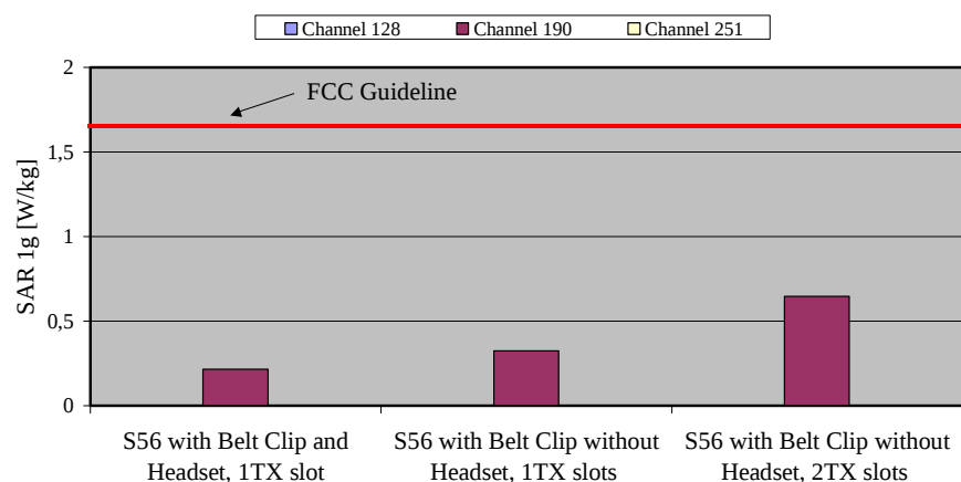
Fig. 11: The measured SAR values in body-worn configuration with Belt Clip (display down) for the Siemens S56 for GSM 850 in comparison to the FCC exposure limit.
