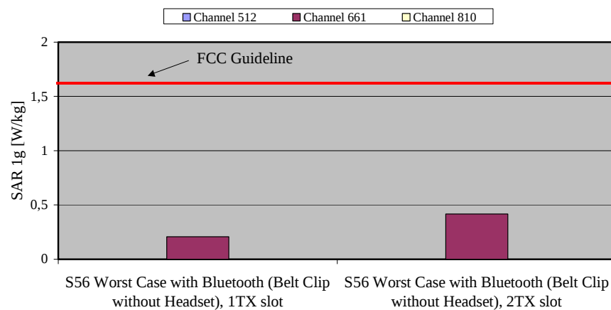
Fig. 18: The measured Worst case SAR values in body-worn configuration with Bluetooth transmitter for the Siemens S56 for PCS 1900 in comparison to the FCC exposure limit.
