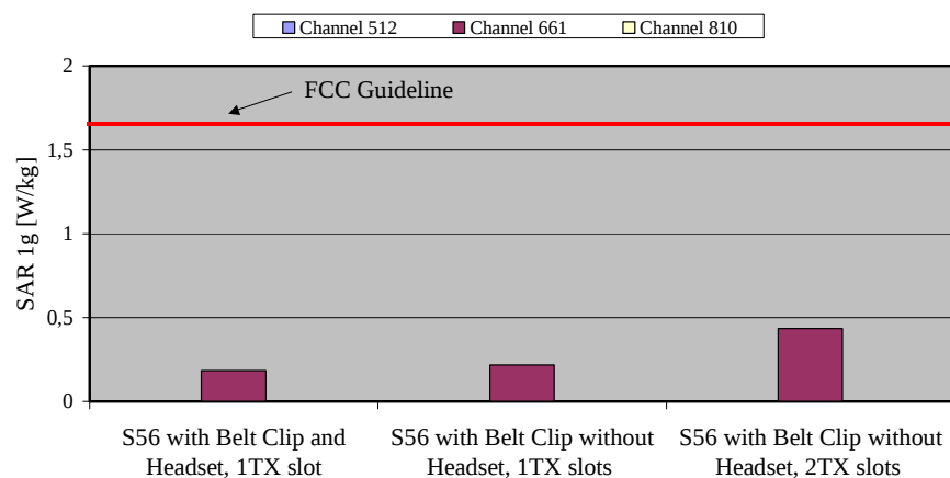
Fig. 15: The measured SAR values in body-worn configuration with Belt Clip (display down) for the Siemens S56 for PCS 1900 in comparison to the FCC exposure limit.
