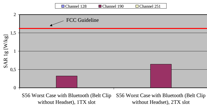
Fig. 14: The Worst Case SAR values in body-worn configuration with Bluetooth transmitter for the Siemens S56 for GSM 850 in comparison to the FCC exposure limit.
