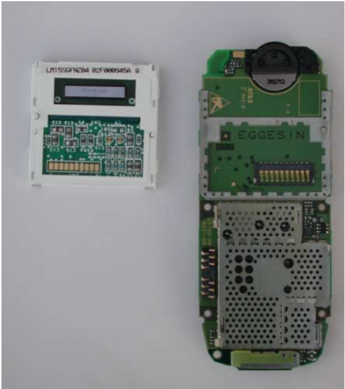
S56 Disassembly step 4
